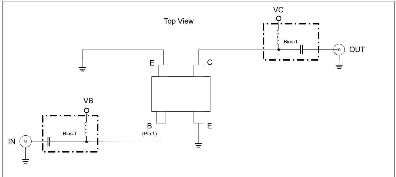
Figure 2 Testing circuit
