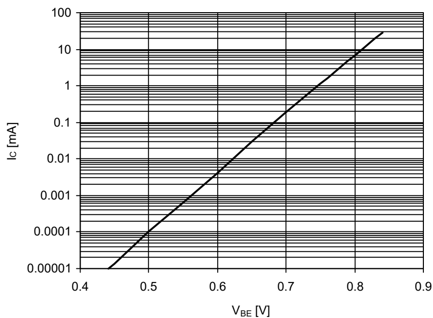
Figure 5 Collector current vs. base emitter forward voltage I_C = f(V_{BE}) , V_{CE} = 2 V
