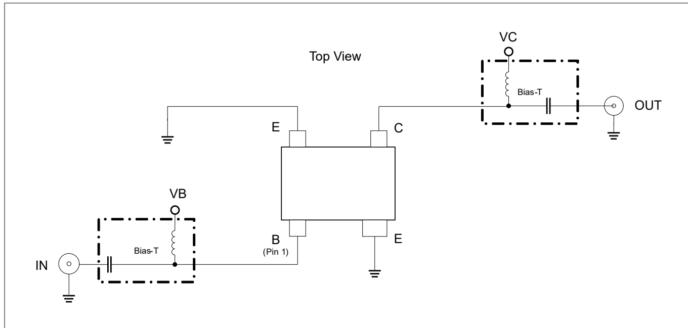
Figure 2 Testing circuit
