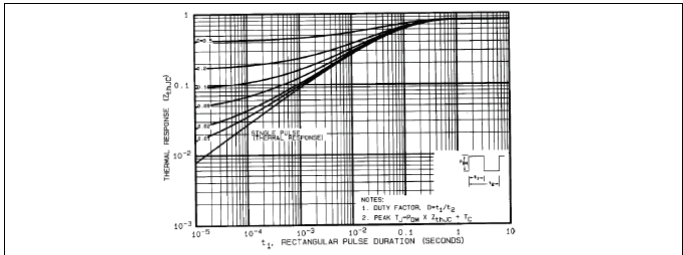
Figure 12 Maximum Effective Transient Thermal Impedance, Junction-to-Case
