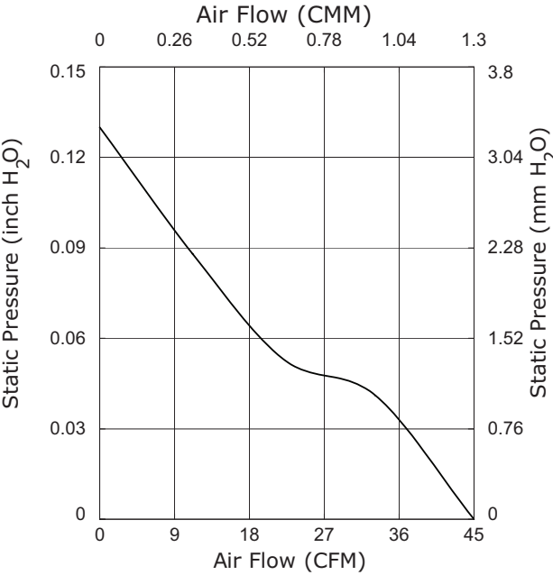
CFM-9225V-127-320
