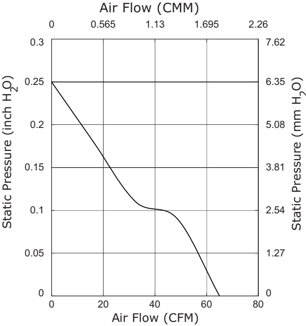
CFM-9225V-145-455
