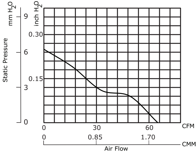
CFM-9225V-339-420
