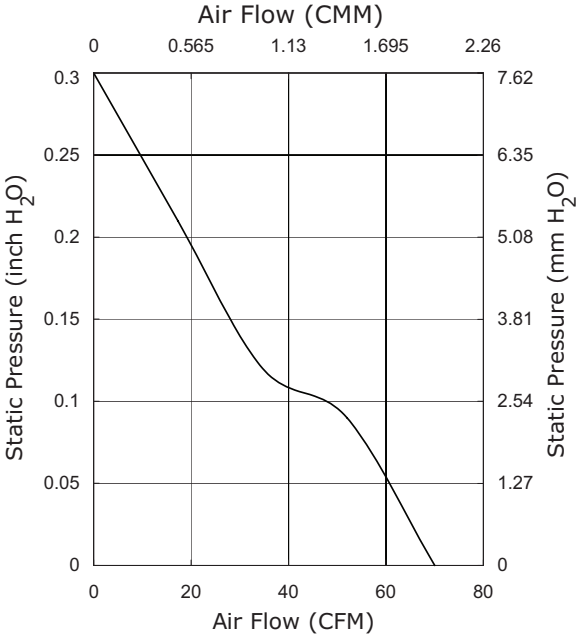
CFM-9225V-224-280
