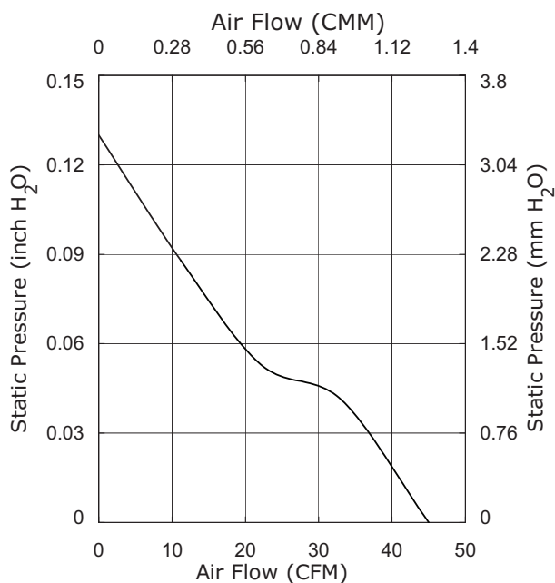
CFM-9225V-239-420
