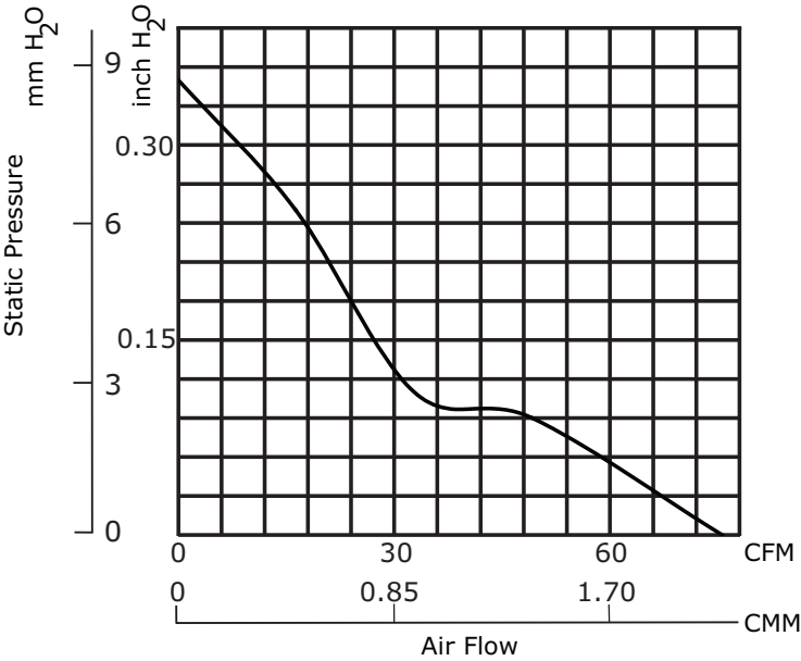
CFM-9225V-245-460
