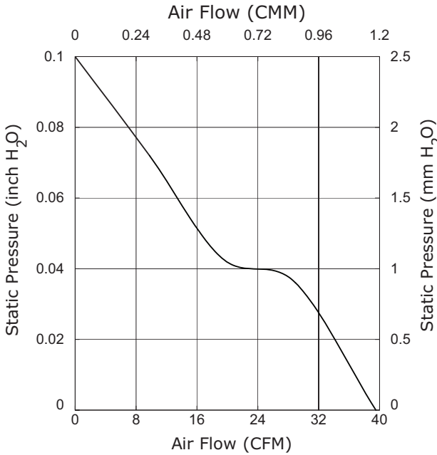
CFM-9225V-124-280
