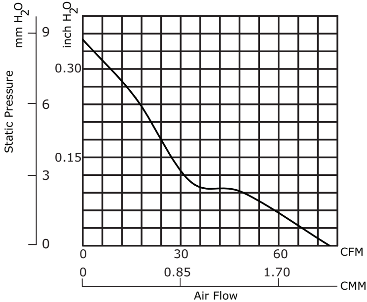
CFM-9225V-345-460
