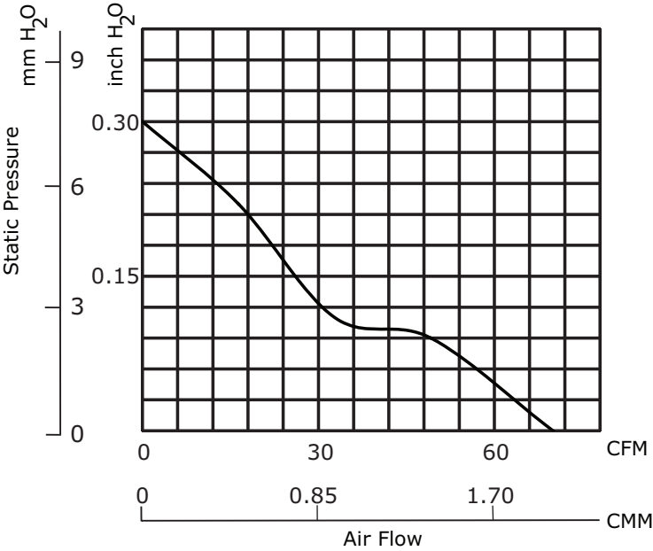
CFM-9225V-342-440
