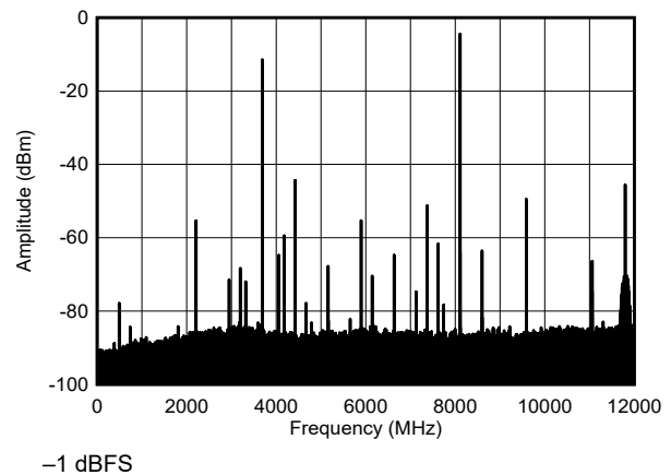
Figure 4-203. TX Single Tone Output Spectrum at 8.11 GHz
