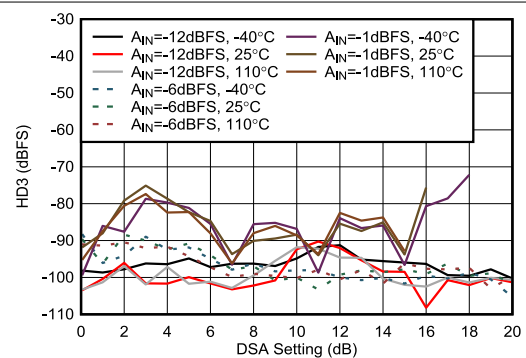
Figure 4-455. RX HD3 vs DSA Setting at 8.1GHz
