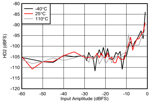
Figure 4-452. RX HD2 vs Digital Amplitude at 8.1GHz
