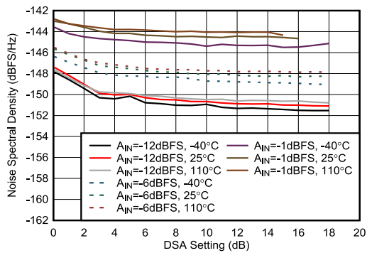
Figure 4-450. RX NSD vs DSA Setting at 8.1GHz
