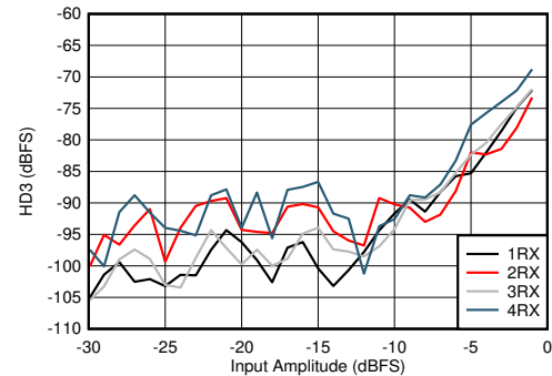
Figure 4-401. RX HD3 vs Input Level and Channel at 3.6 GHz
