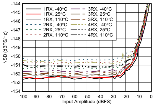
Figure 4-475. RX NSD vs Digital Amplitude at 9.6 GHz
