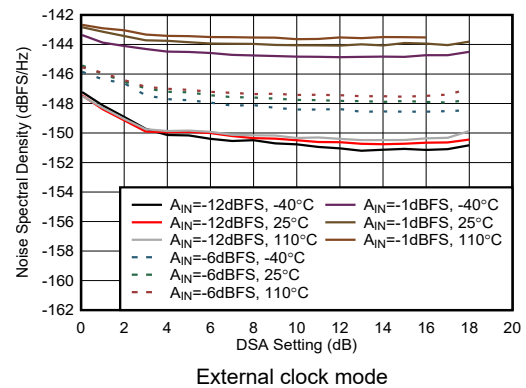
Figure 4-451. RX NSD vs DSA Setting at 8.1GHz
