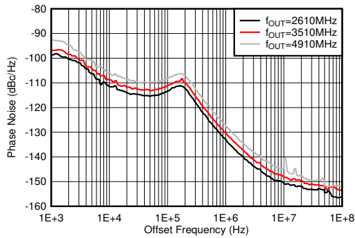
Figure 4-507. Phase Noise for 10-GHz VCO vs Offset Frequency and f_{OUT} at -40^{\circ}\text{C}
