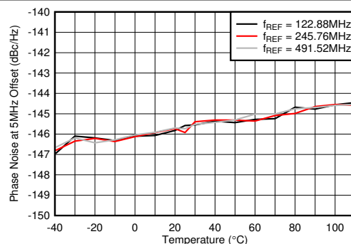
Figure 4-514. Phase Noise for 10-GHz VCO at 5 MHz vs Temperature and f_{REF} at f_{OUT} = 2.6 GHz
