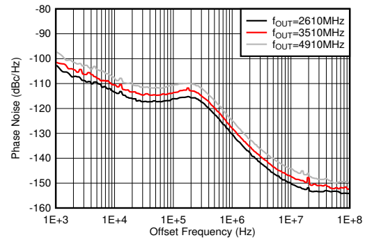
Figure 4-508. Phase Noise for 10-GHz VCO vs Offset Frequency and f_{OUT} at 110^{\circ}\text{C}
