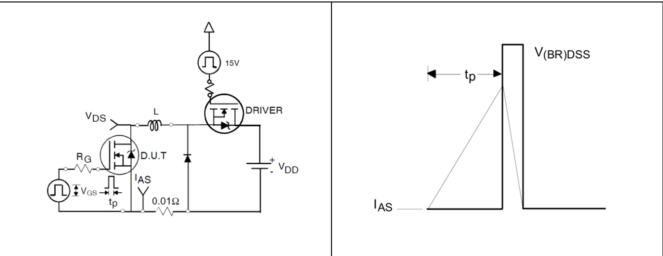
Figure 19 Unclamped Inductive Test Circuit
