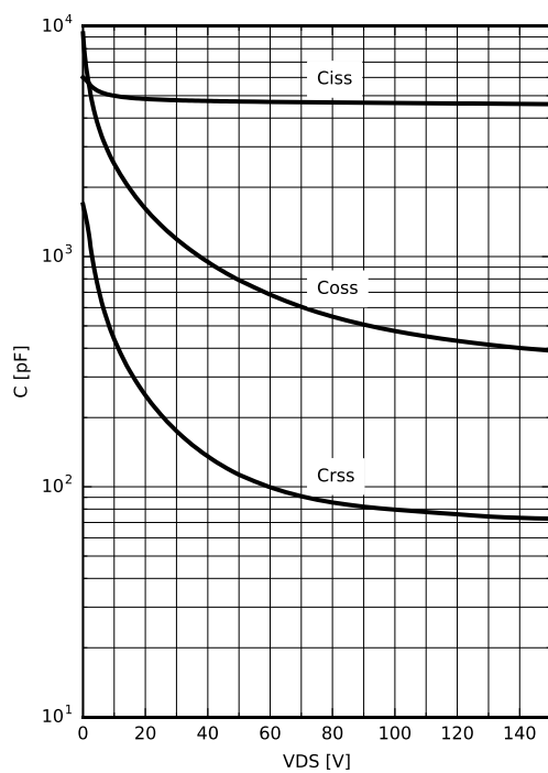
Diagram 11: Typ. capacitances
