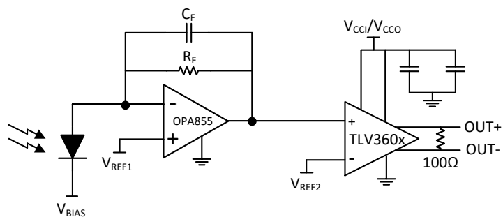
图 8-7. Optical Receiver
