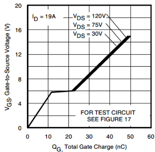
Figure 11 Typical Gate Charge Vs. Typical Gate-to-Source Voltage
