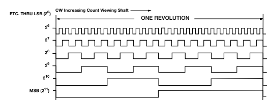
Figure 2 Natural Binary
