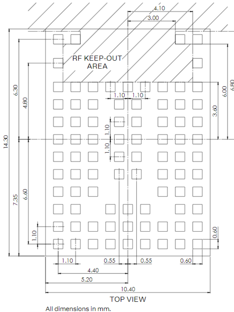
Figure 16: MAYA-W2 footprint
