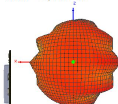
Theta = 90, Phi = 90
