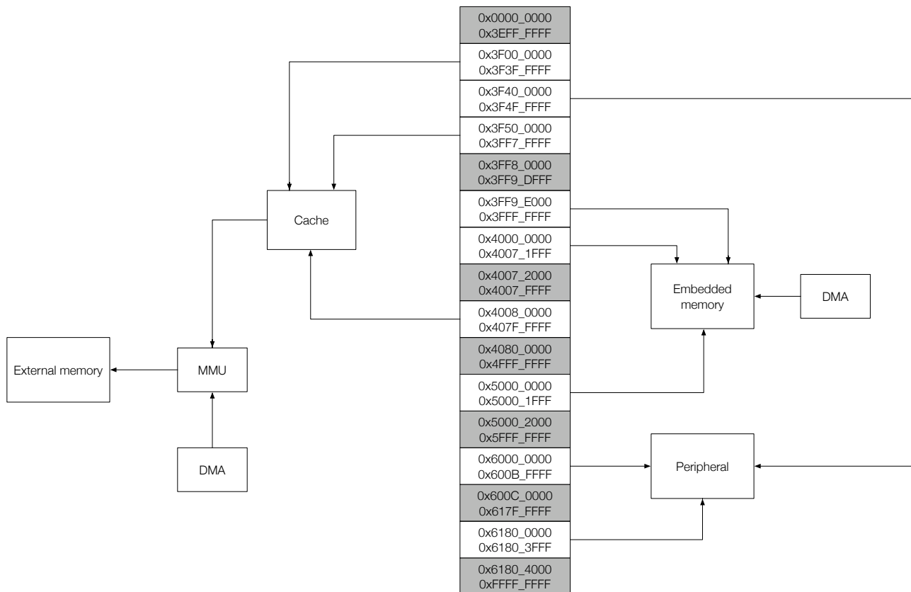
Figure 6: Address Mapping Structure
