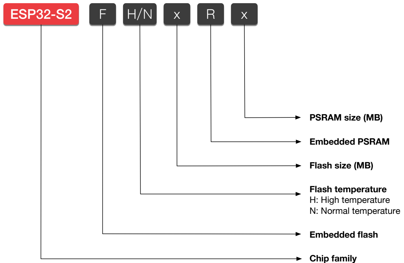
Figure 2: ESP32-S2 Family Nomenclature
