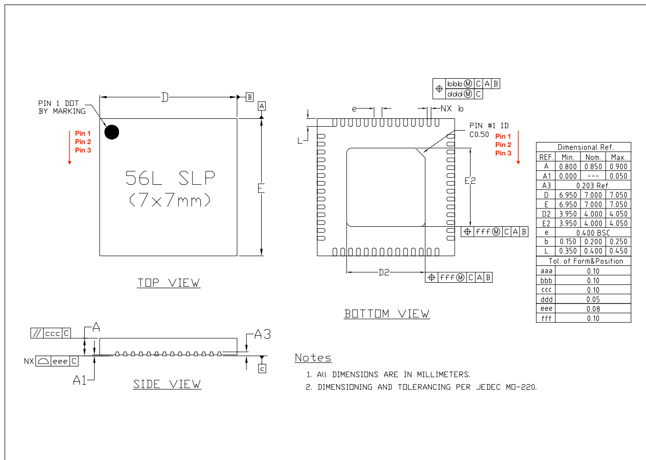
Figure 7: QFN56 (7x7 mm) Package
