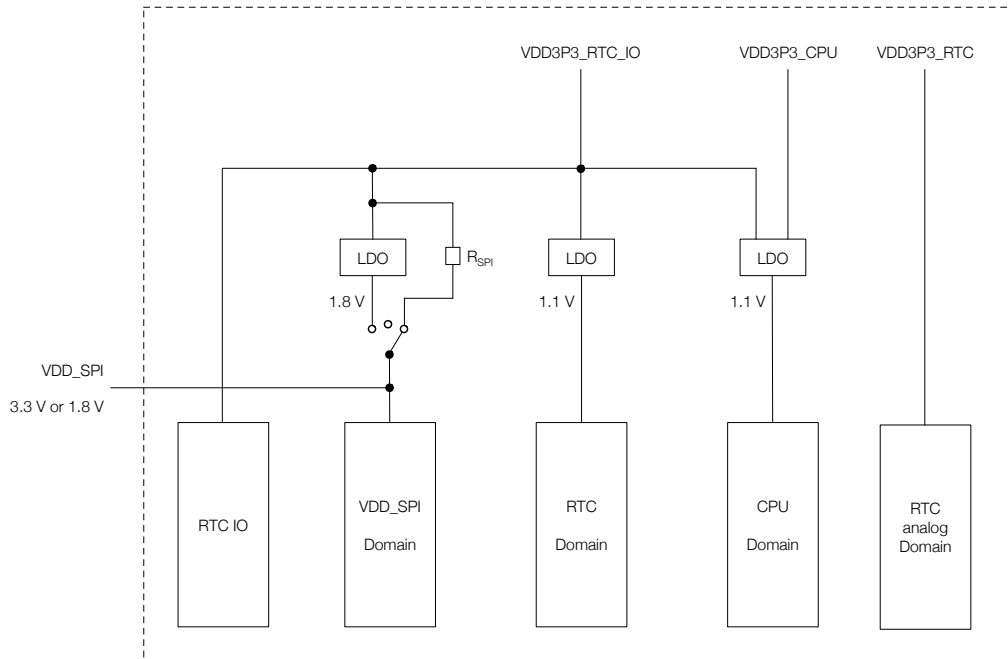
Figure 4: ESP32-S2 Family Power Scheme
