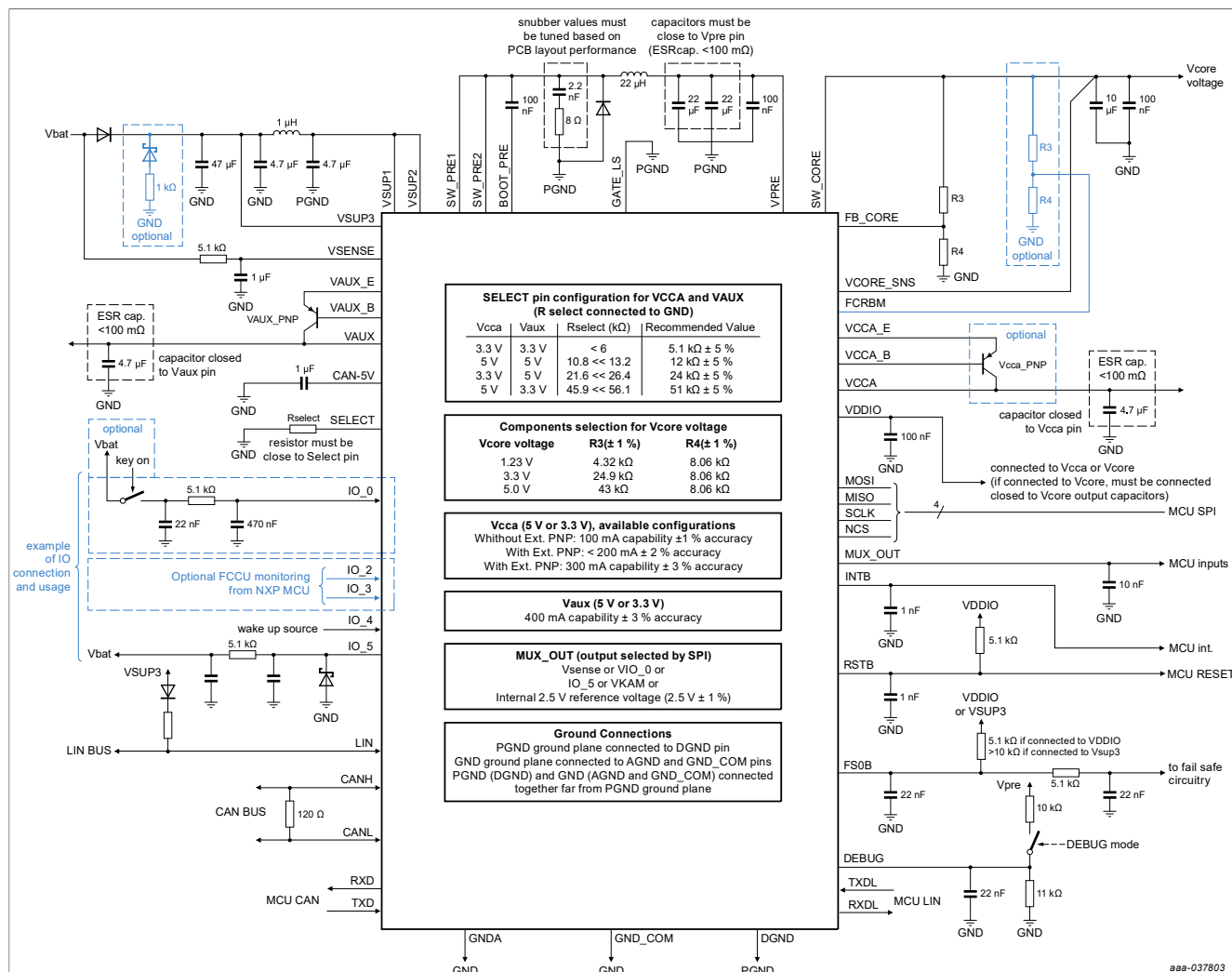
Figure 74. F4500 simplified application schematic with CAN, LIN, IO_5, buck only V_{PRE} configuration
