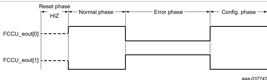
Figure 13. IO_2:3 MCU error monitoring: bi-stable protocol
