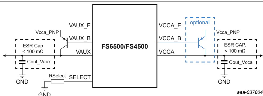
Figure 75. V AUX /V CCA connection, deep fail-safe enabled
