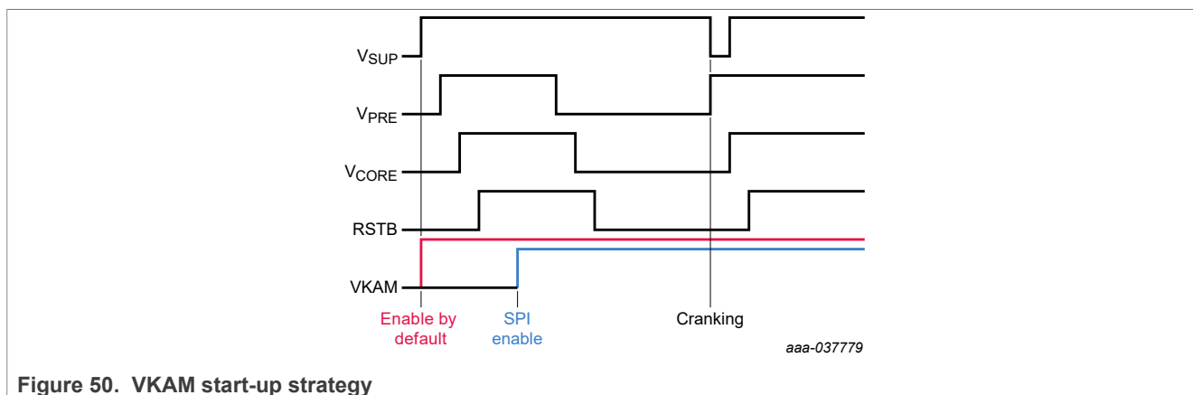
Figure 50. VKAM start-up strategy
