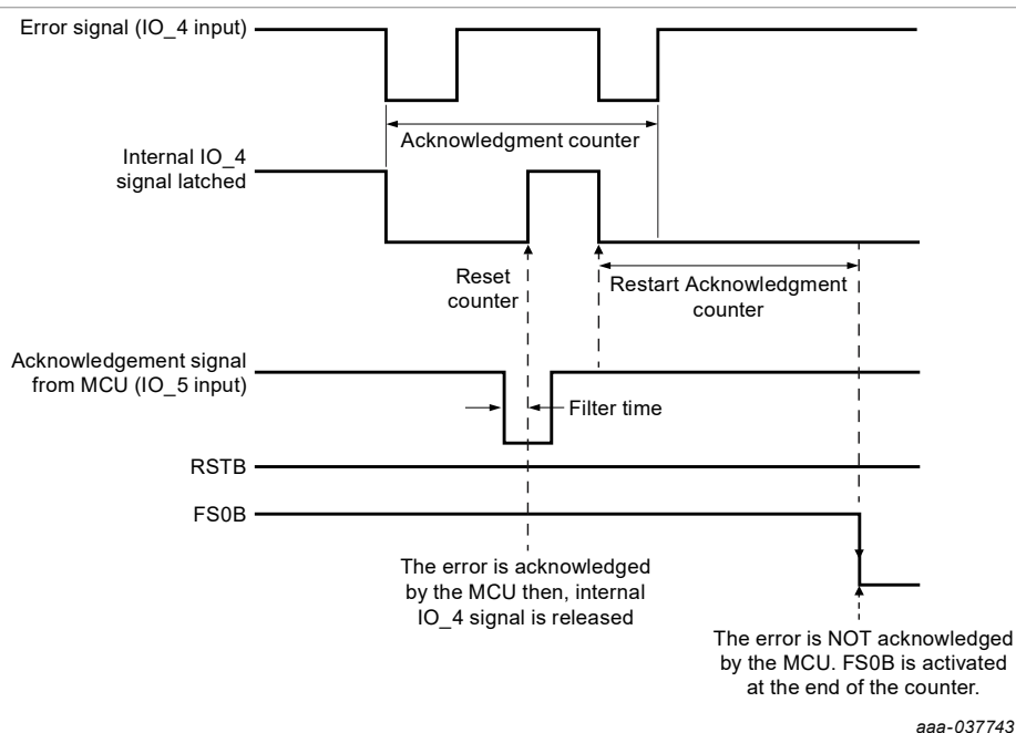
Figure 14. External error signal handling
