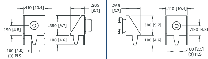
Mounting Detail for Two Contacts
