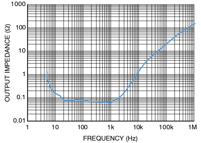
Figure 18. Buffer Output Impedance vs. Frequency
