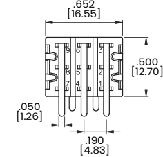
P.C.MOUNTING
