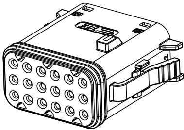
18CCT PLUG CONNECTOR WITHOUT HEATSHRINK HOUSING
