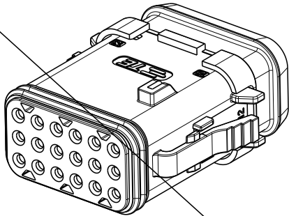
18CCT PLUG CONNECTOR WITH HEATSHRINK HOUSING
