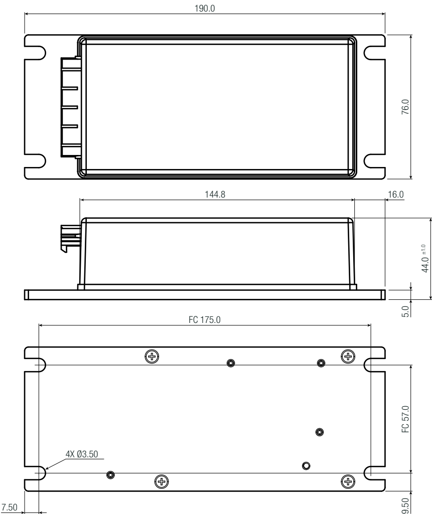
MOLEX Connector without CRTL function "/MO"
