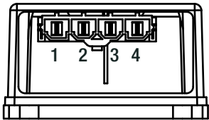
MOLEX Connector without CRTL function "/MO"
