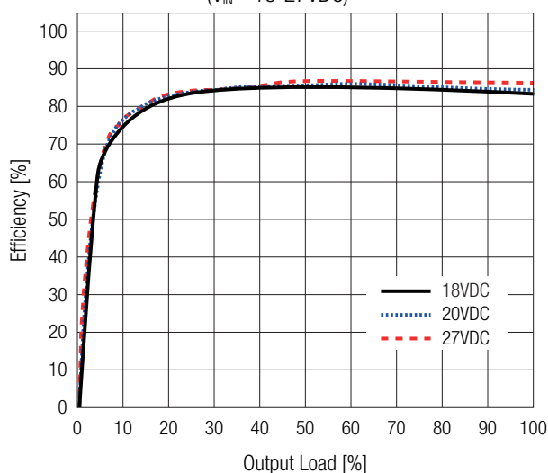
Efficiency vs. Load ( V_{IN} = 18-27\text{VDC} )
