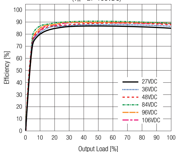
Efficiency vs. Load ( V_{IN} = 27-106\text{VDC} )
