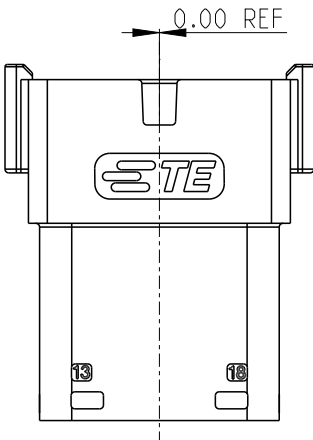
KEYING OPTION C
