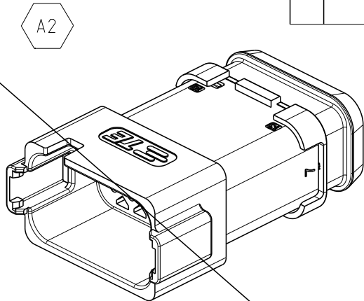
18CCT RECEPTACLE CONNECTOR WITH HEATSHRINKING HOUSING
