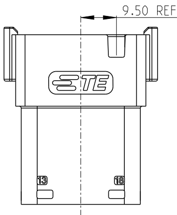
KEYING OPTION A
