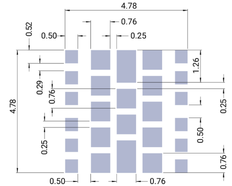
Recommended Stencil Opening
