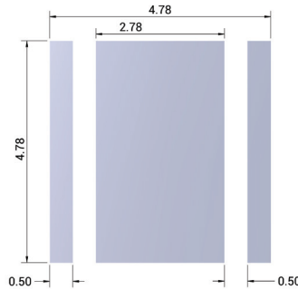
Recommended Solder Mask Opening
