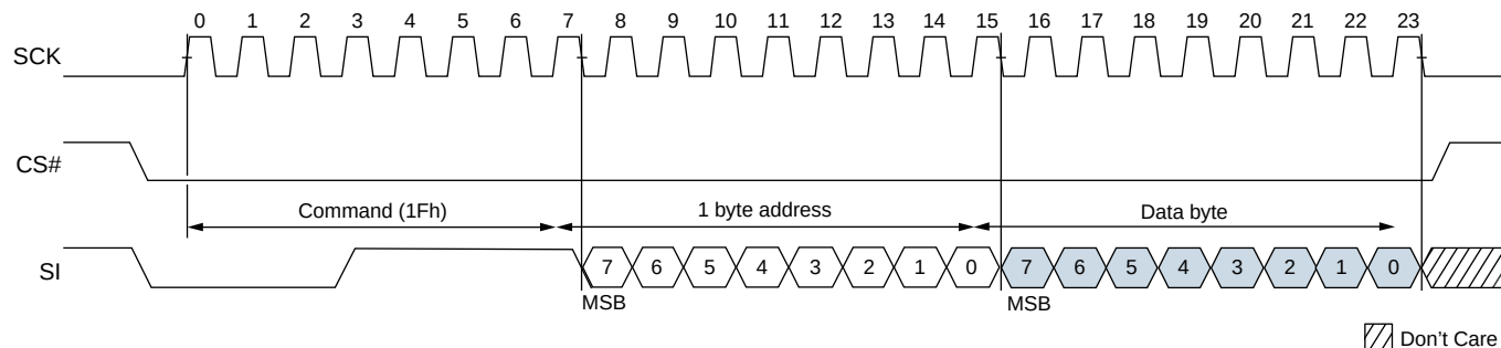
Figure 25: SET FEATURE (1Fh) Timing
