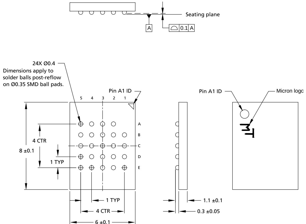
Figure 36: 24-Pin T-PBGA (5 x 5 Ball Grid Array) 6mm x 8mm – Package Code: 12
