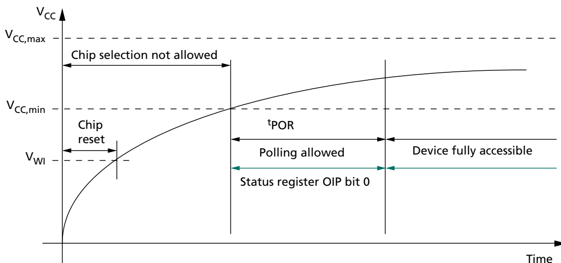
Figure 29: SPI Power-Up
