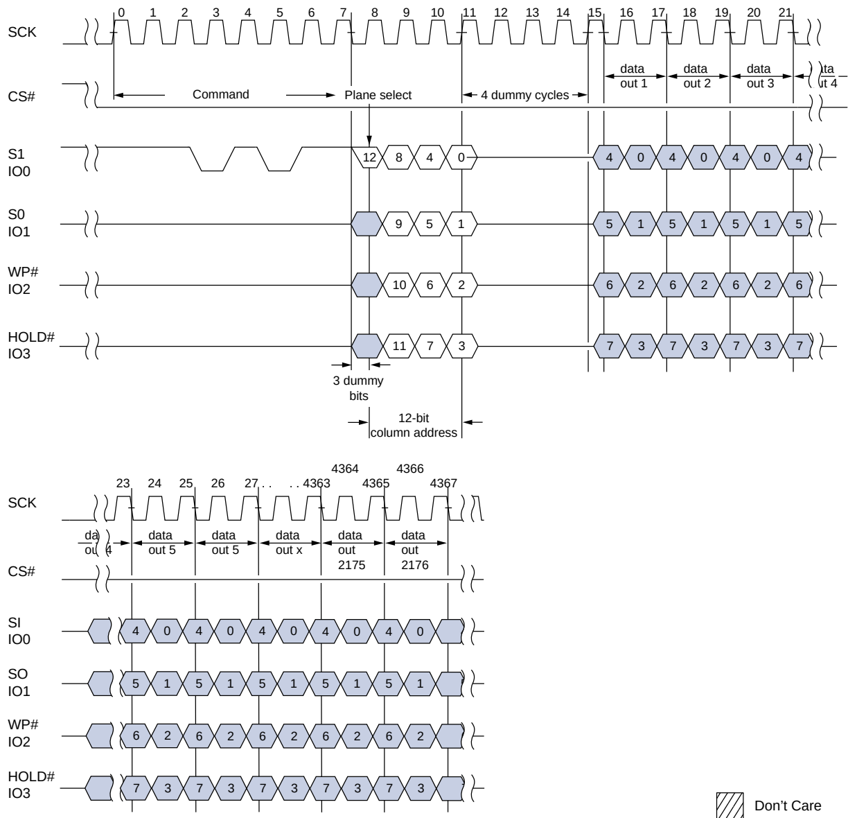
Figure 16: READ FROM CACHE Quad I/O
