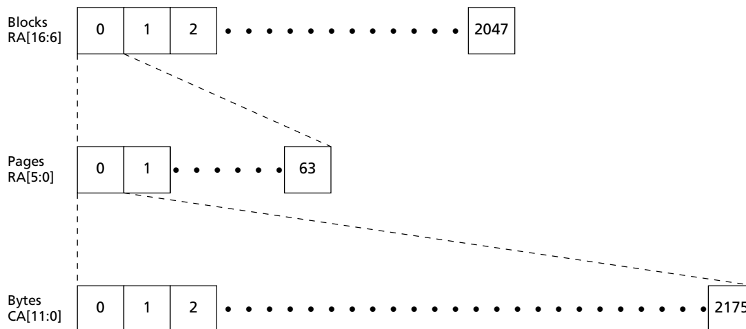
Figure 5: Memory Map
