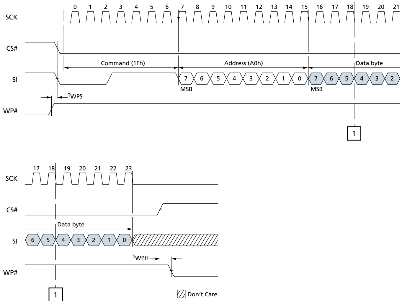
Figure 33: Serial Input Timing
