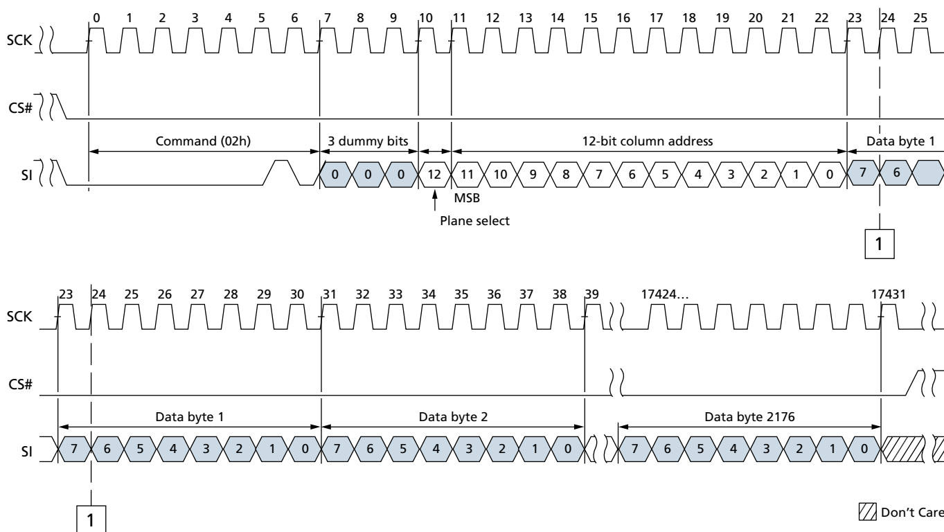
Figure 19: PROGRAM LOAD (02h) Timing
