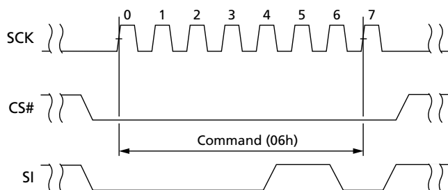
Figure 9: WRITE ENABLE (06h) Timing
