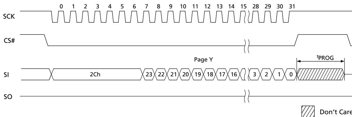
Figure 26: PROTECT Command Cycle
