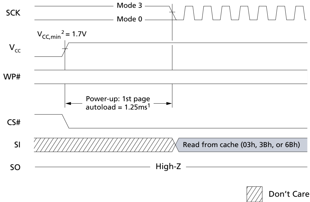
Figure 30: Automatic Device Initialization
