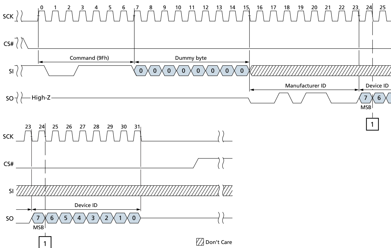
Figure 18: READ ID (9Fh) Timing
