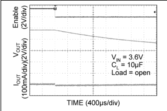
FIGURE 2-30: MIC94081 Scope 6.
