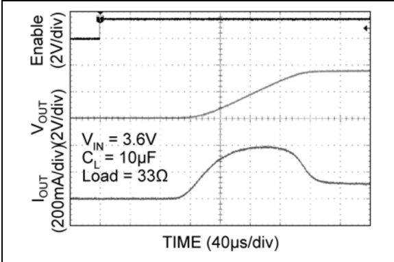
FIGURE 2-54: MIC94084 Scope 8.
