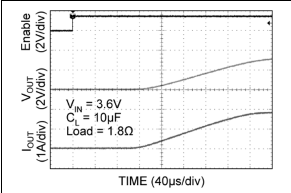
FIGURE 2-52: MIC94084 Scope 6.
