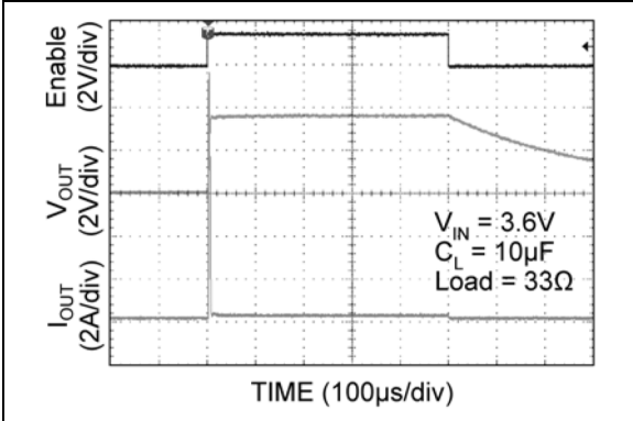
FIGURE 2-28: MIC94081 Scope 4.
