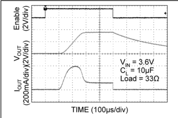
FIGURE 2-53: MIC94084 Scope 7.
