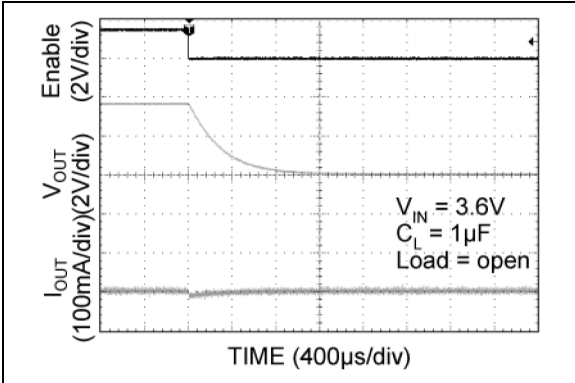
FIGURE 2-29: MIC94081 Scope 5.
