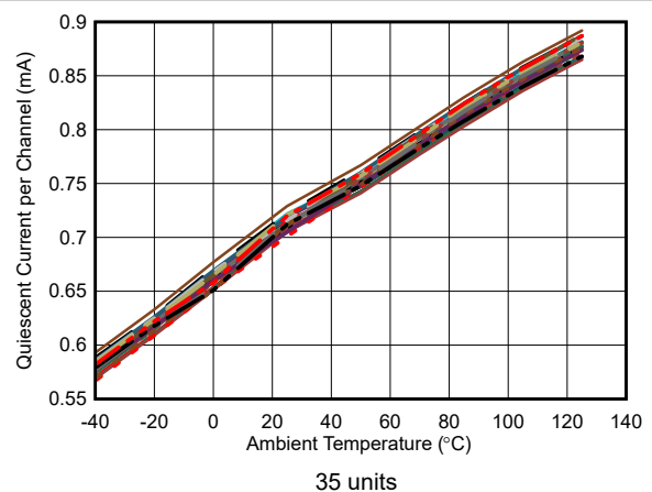
图 7-24. Quiescent Current vs Ambient Temperature
