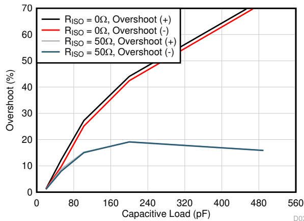
图 7-5. Small-Signal Overshoot vs Capacitive Load (20-mV pp Output Step, G = +1)
