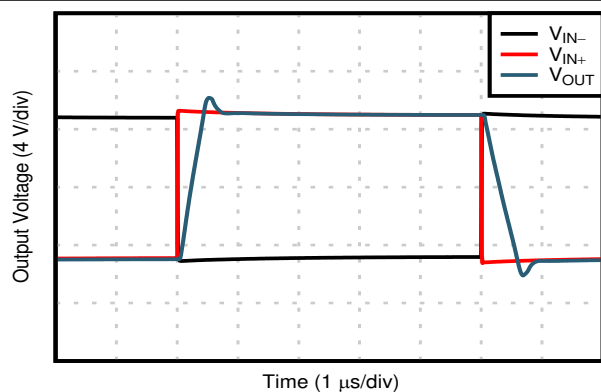
Figure 7-43. Settling Time
