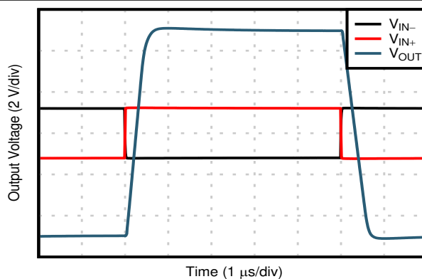
Figure 7-44. Settling Time
