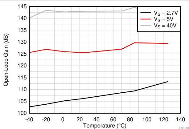
图 6-24. Open-Loop Voltage Gain vs Temperature (dB)
