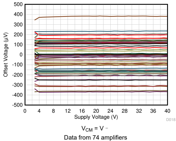
图 6-7. Offset Voltage vs Power Supply
