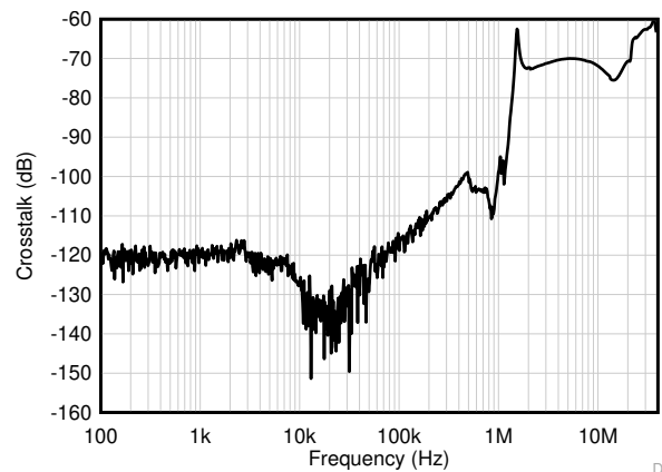
图 6-36. Channel Separation vs Frequency
