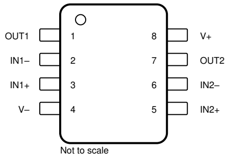
图 5-3. TLV9362-Q1 D and DGK Package, 8-Pin SOIC and VSSOP (Top View)
