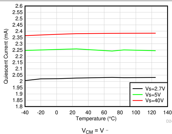
图 6-23. Quiescent Current vs Temperature
