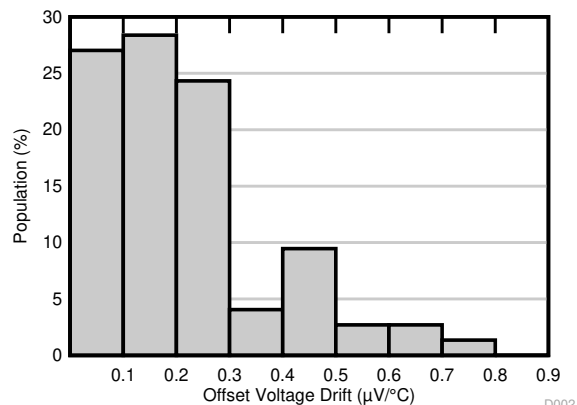
图 6-2. Offset Voltage Drift Distribution
