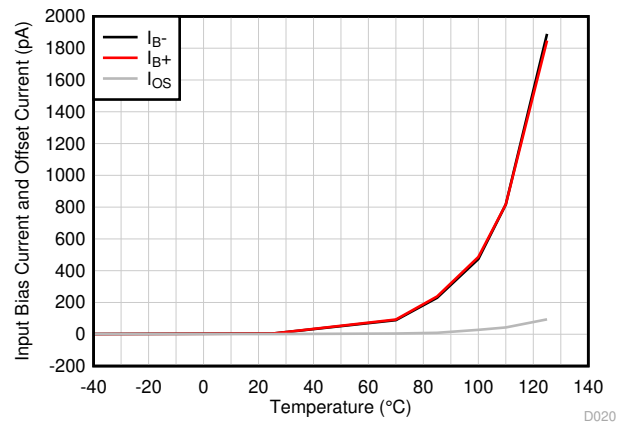
图 6-10. Input Bias Current and Offset Current vs Temperature
