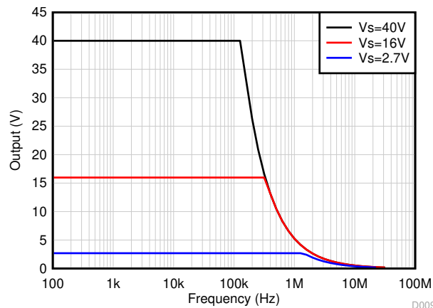
图 6-35. Maximum Output Voltage vs Frequency
