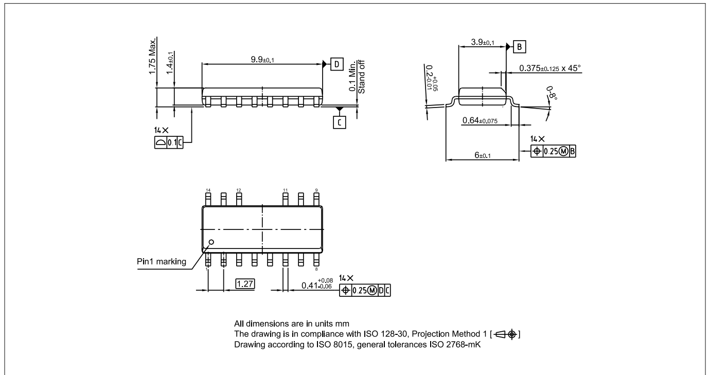
Figure 24 DSO14-150mil outline
