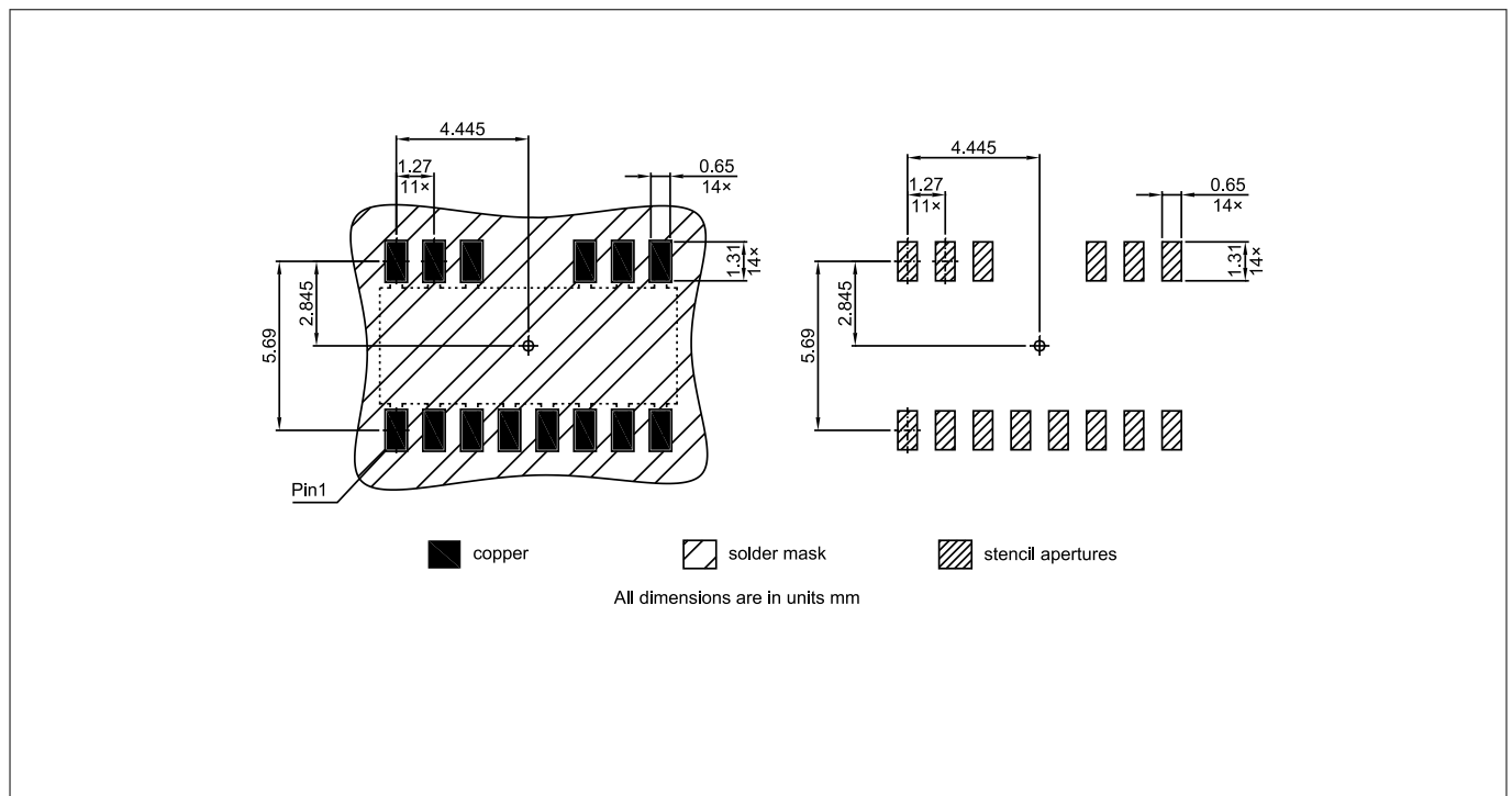
Figure 25 DSO14-150mil footprint
