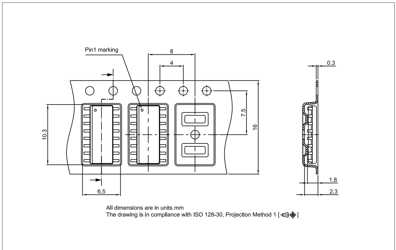
Figure 23 DSO16-150mil packing
