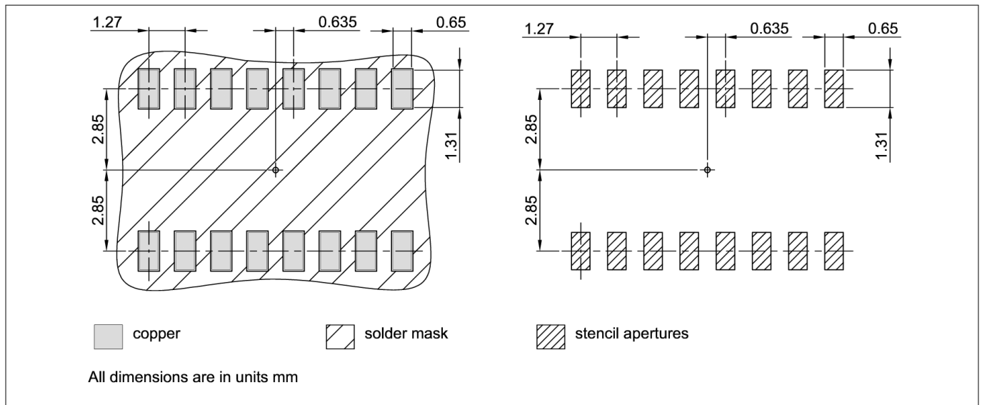
Figure 22 DSO16-150mil footprint
