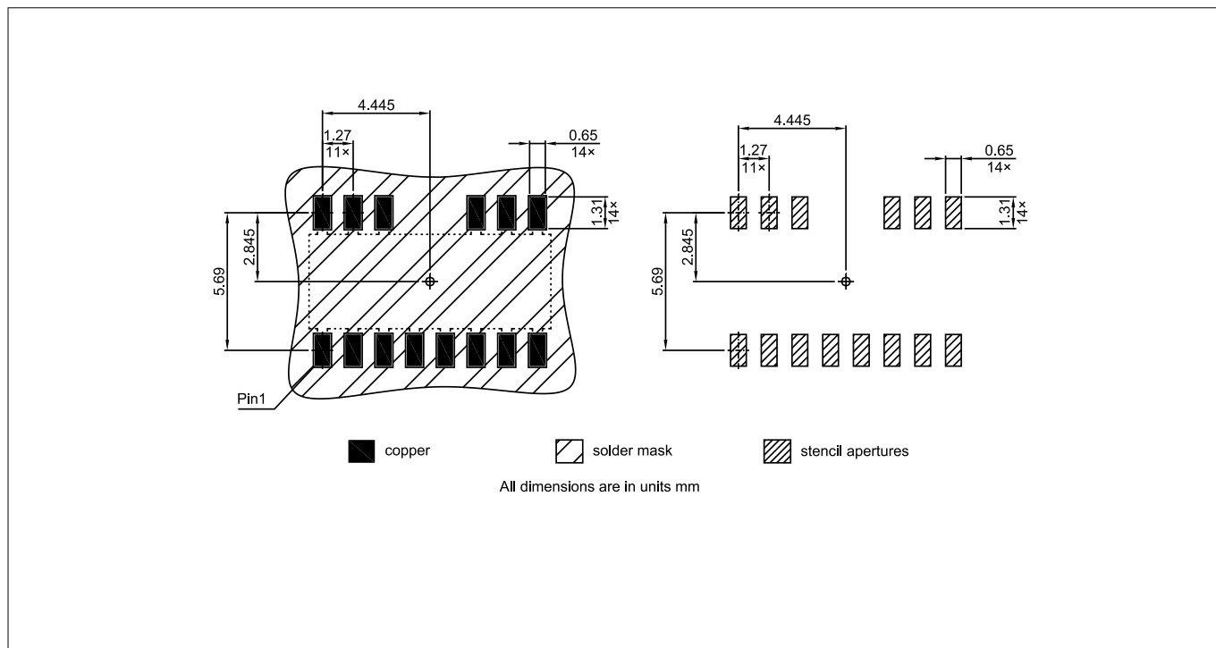
Figure 25 DSO14-150mil footprint
