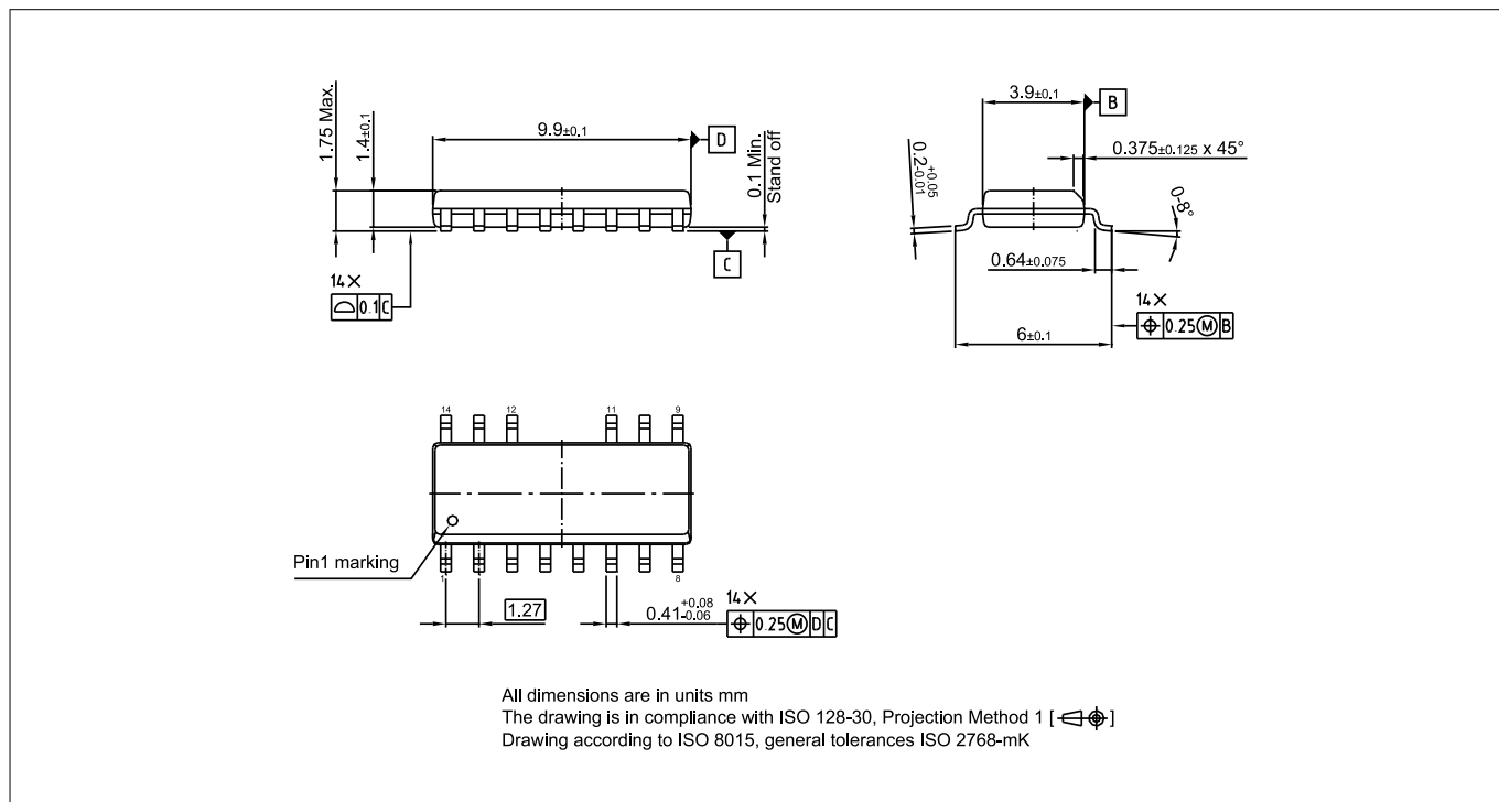
Figure 24 DSO14-150mil outline
