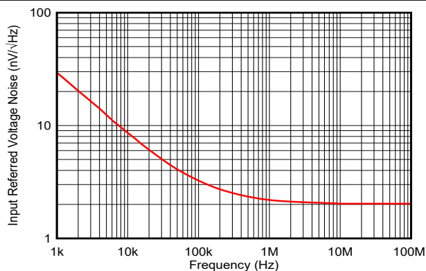
图 6-8. Voltage Noise Density vs Frequency
