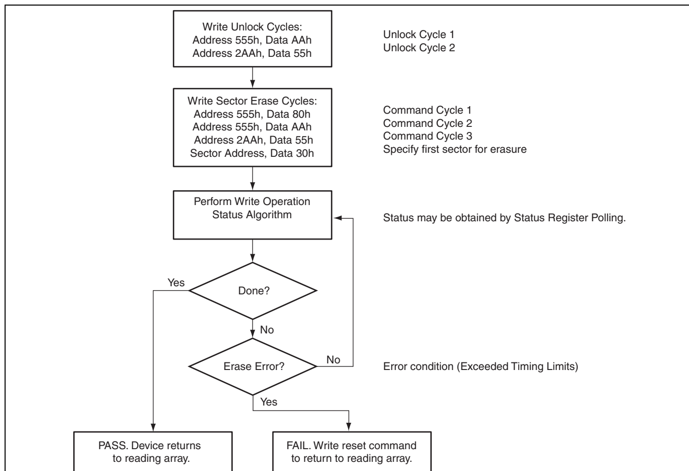
Figure 37 Sector erase operation
