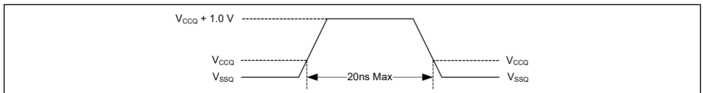
Figure 53 Maximum positive overshoot waveform
