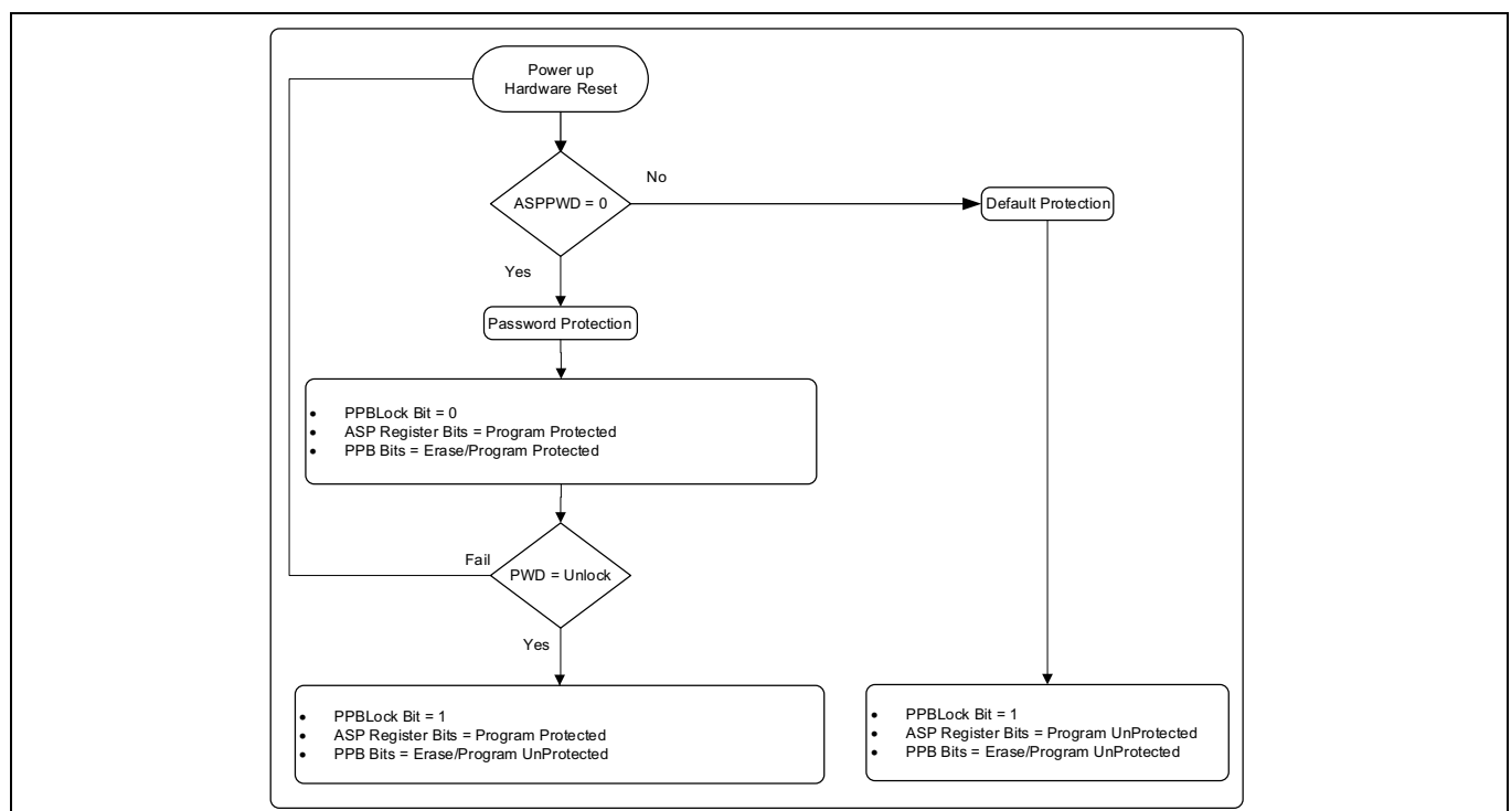
Figure 29 Password protection scheme flowchart
