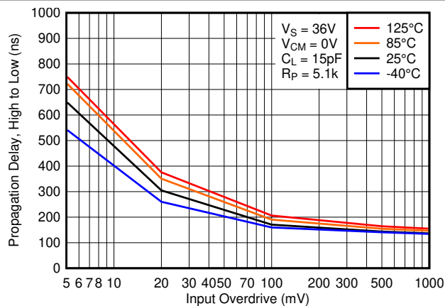
图 6-32. High to Low Propagation Delay vs. Input Overdrive Voltage, 36V
