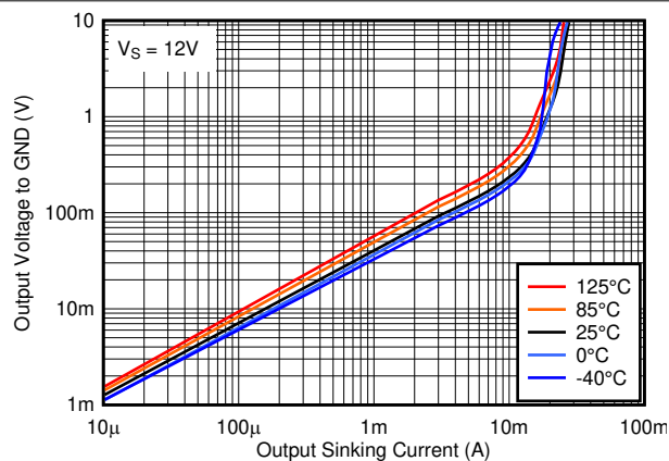
图 6-24. Output Low Voltage vs. Output Sinking Current at 12V
