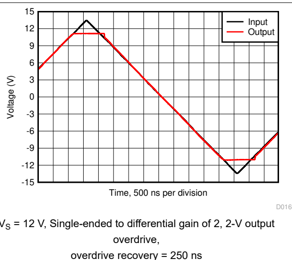
图 10-5. Overdrive Recovery Performance
