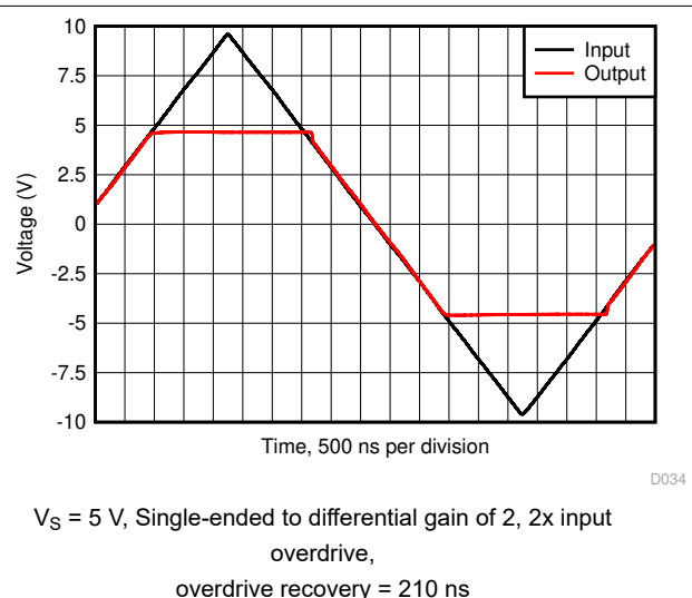
图 10-6. Overdrive Recovery Performance
