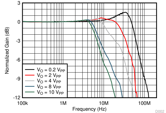
图 7-2. Frequency Response vs V_O
