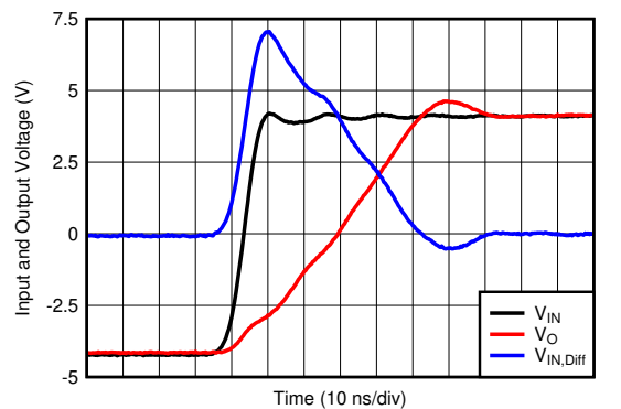
图 9-18. Large-Signal Transient Response Using the OPA810
