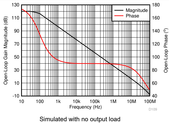
图 7-42. Open-Loop Gain and Phase vs Frequency
