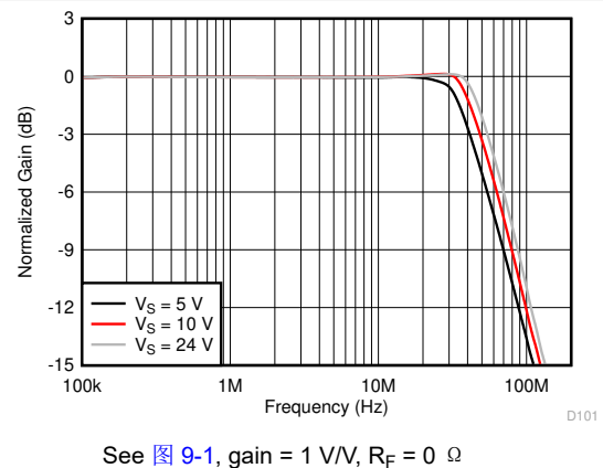
图 7-43. Large-Signal Response vs Supply Voltage
