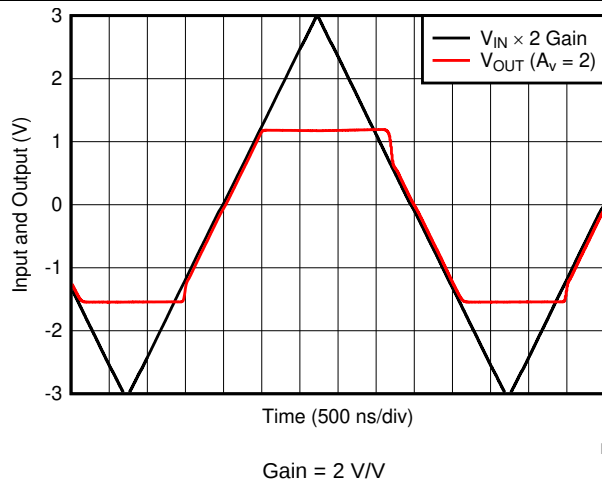
图 23. Noninverting Overdrive Recovery
