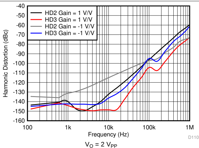
图 11. Harmonic Distortion vs Frequency
