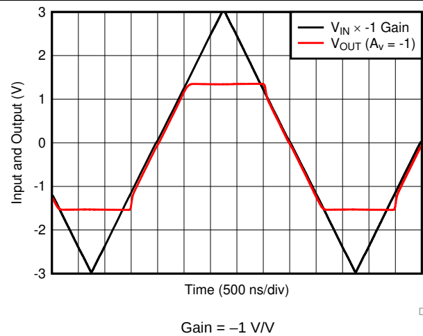
图 24. Inverting Overdrive Recovery
