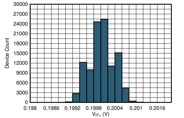
TLV40x1R2 图 7-8. Positive Threshold Histogram V_S = 5\text{ V}
