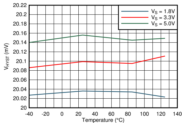
TLV40x1R2 图 7-11. Hysteresis vs Temperature
