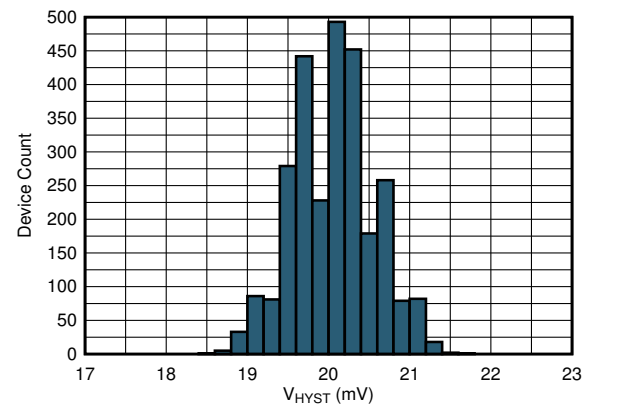
TLV40x1R2 图 7-12. Hysteresis Histogram V_S = 5\text{ V}
