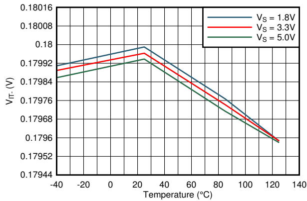
TLV40x1R2 图 7-9. Negative Threshold vs Temperature
