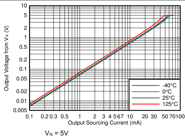
图 7-26. Output Voltage vs Output Sourcing Current
