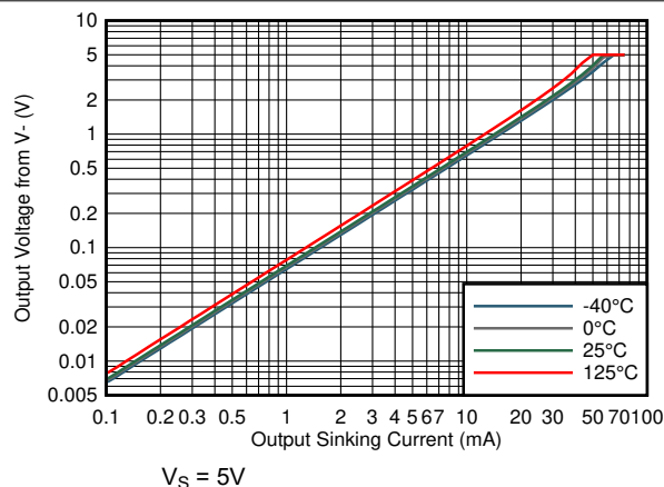
图 7-25. Output Voltage vs Output Sinking Current
