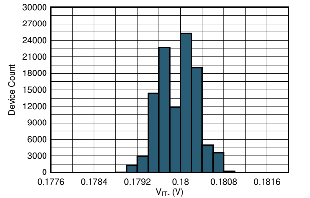
TLV40x1R2 图 7-10. Negative Threshold Histogram V_S = 5\text{ V}
