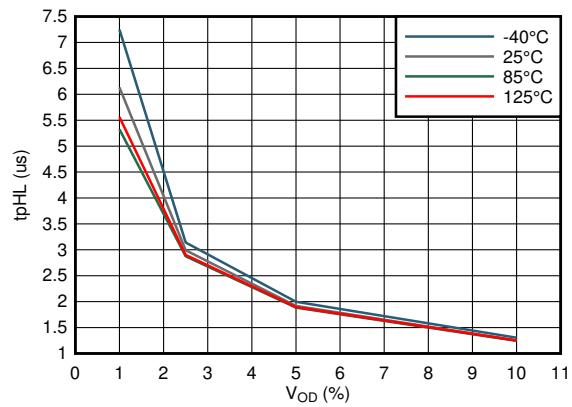
图 7-31. Propagation Delay High-Low vs Input Overdrive
