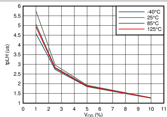
图 7-28. Propagation Delay Low-High vs Input Overdrive
