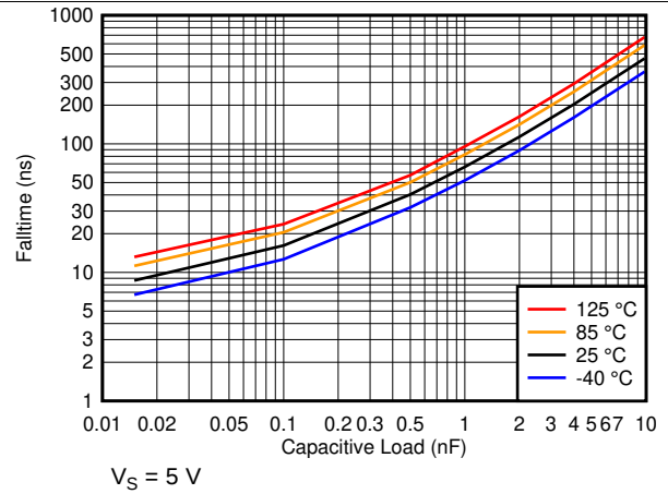
图 54. t_{\text{FALL}} vs. Capacitive Load at 5V
