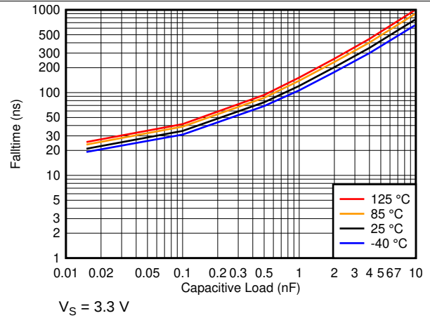
图 52. t_{\text{FALL}} vs. Capacitive Load at 3.3V
