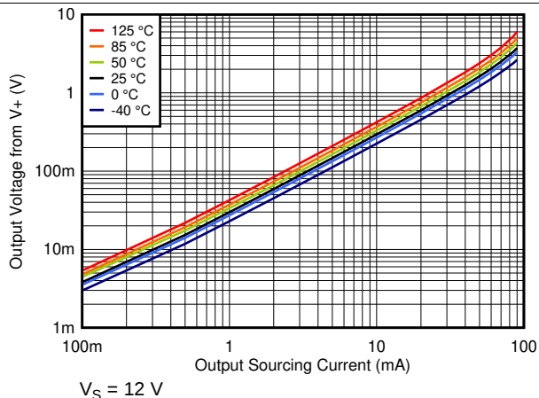
图 28. Output Voltage vs. Output Sourcing Current at 12V
