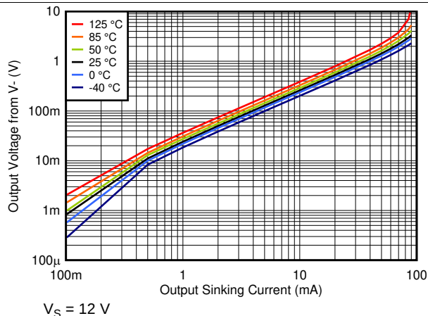
图 27. Output Voltage vs. Output Sinking Current at 12V
