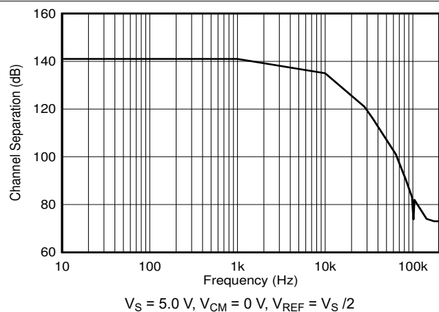
图 6-42. Channel Separation vs. Frequency (INA2191)
