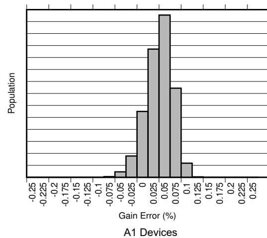
图 6-6. Gain Error Production Distribution (INA2191)
