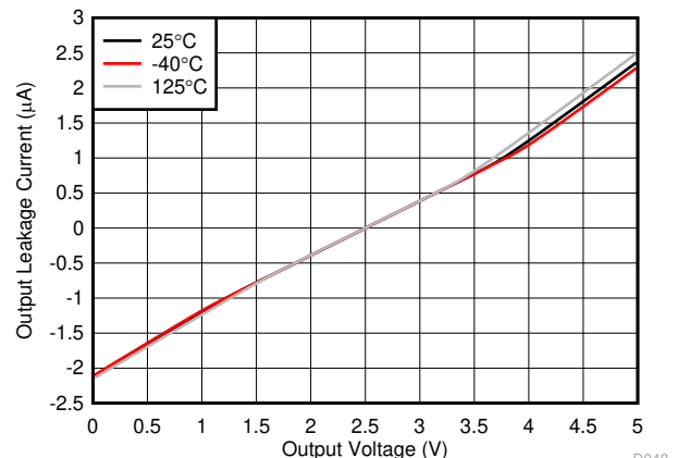
图 6-38. Output Leakage vs. Output Voltage
