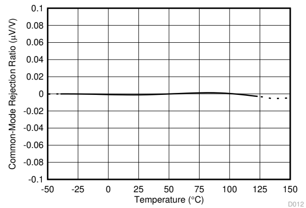
图 6-4. Common-Mode Rejection Ratio vs. Temperature
