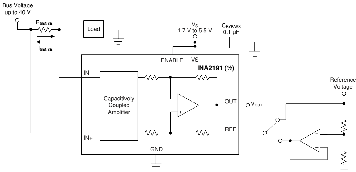
图 7-6. Bidirectional Application
