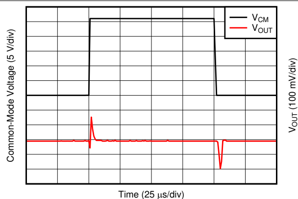
图 5-28. Common-Mode Voltage Transient Response
