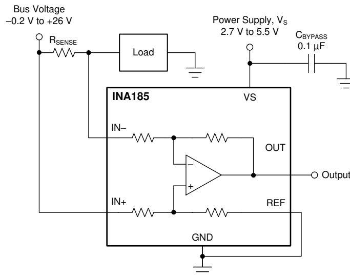
图 6-2. Unidirectional Application
