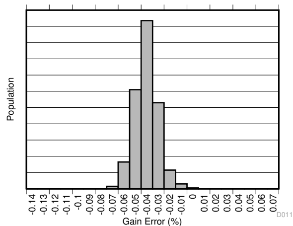
图 5-11. Gain Error Production Distribution A1
