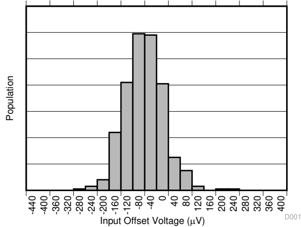
图 5-1. Input Offset Voltage Production Distribution A1
