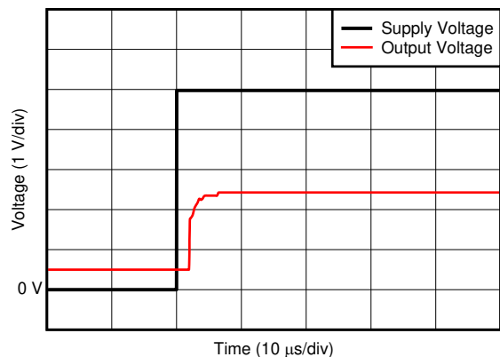
图 5-31. Start-Up Response
