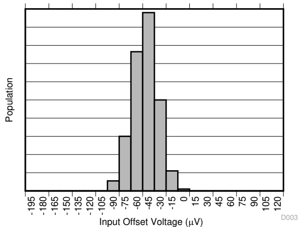
图 5-3. Input Offset Voltage Production Distribution A3
