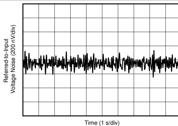
图 5-26. 0.1-Hz to 10-Hz Voltage Noise (Referred-to-Input)
