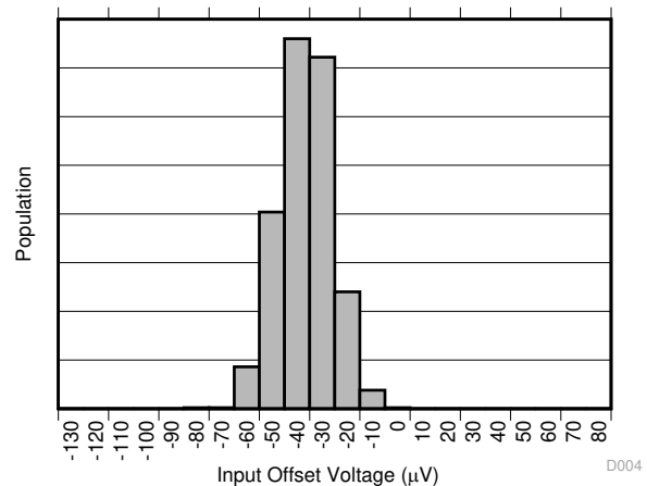
图 5-4. Input Offset Voltage Production Distribution A4
