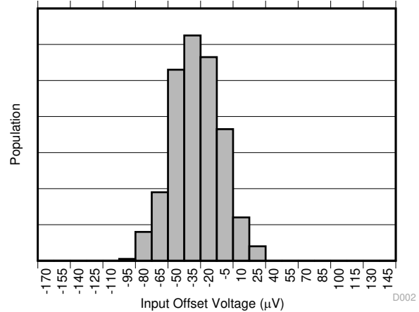
图 5-2. Input Offset Voltage Production Distribution A2
