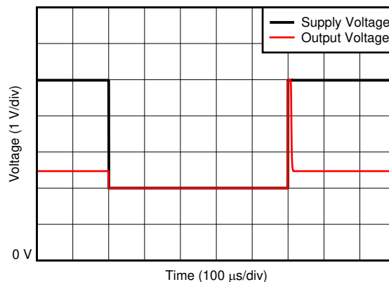
图 5-32. Brownout Recovery
