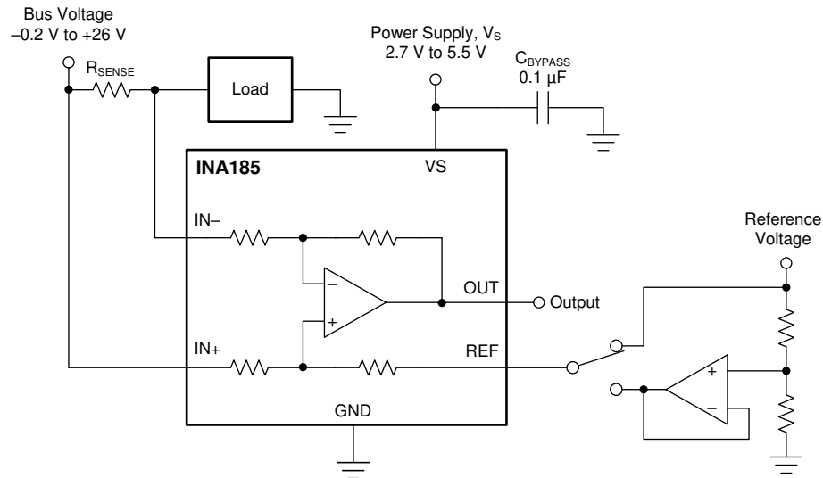
图 6-3. Bidirectional Application
