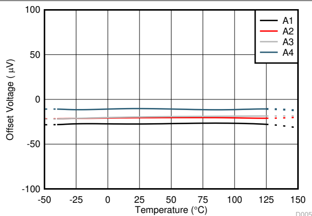
图 5-5. Offset Voltage vs Temperature
