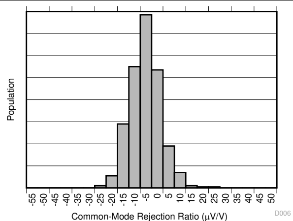
图 5-6. Common-Mode Rejection Production Distribution A1
