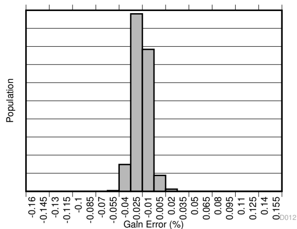
图 5-12. Gain Error Production Distribution A2
