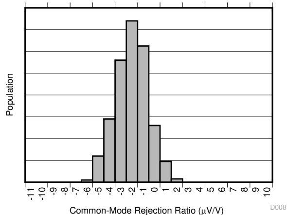
图 5-8. Common-Mode Rejection Production Distribution A3
