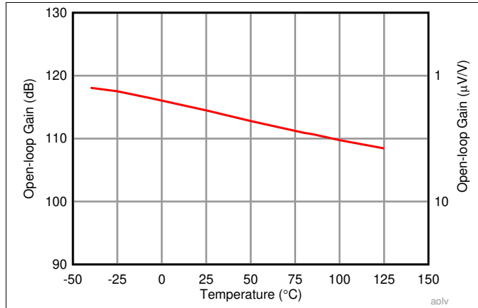
图 19. Open-Loop Gain vs Temperature
