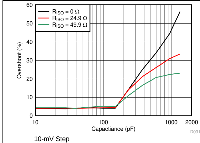
图 21. Small-Signal Overshoot vs Capacitive Load
