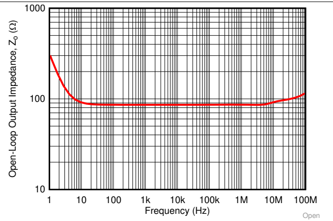
图 20. Open-Loop Output Impedance vs Frequency
