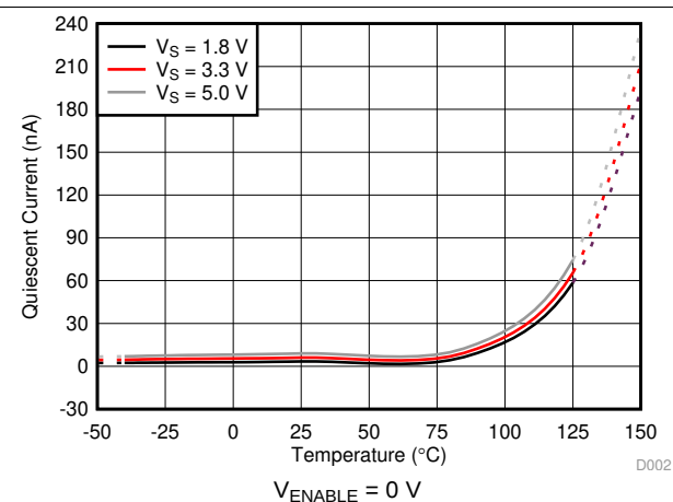
图 18. Quiescent Current vs Temperature (Disabled)
