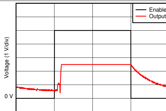
图 26. Start-Up Response
