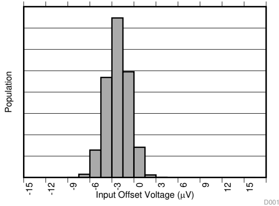
图 1. Input Offset Voltage Production Distribution
