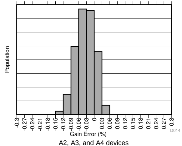
图 6. Gain Error Production Distribution
