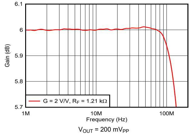
图 7-4. 0.1-dB Gain Flatness Frequency Response
