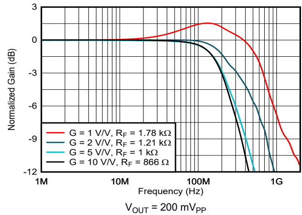
图 7-2. Noninverting Small-Signal Frequency Response
