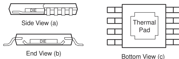
图 9-6. Views of Thermal Enhanced Package
