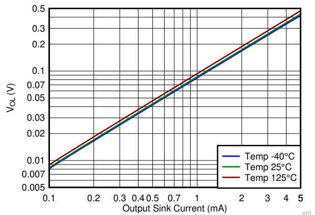
图 6-21. Output Voltage Low vs Output Sink Current
