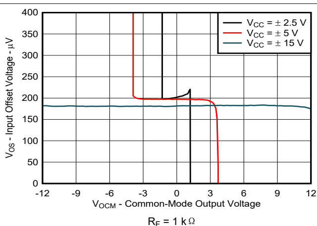
图 7-26. Input Offset Voltage vs Common-Mode Output Voltage
