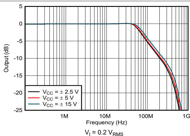
图 7-7. Large-Signal Frequency Response
