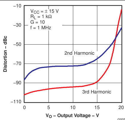
图 5-34. Distortion vs Output Voltage
