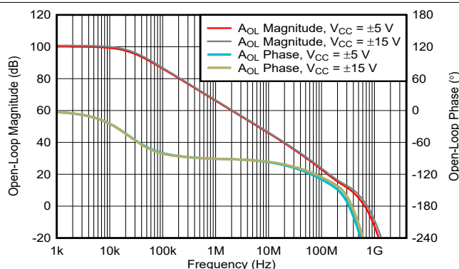
图 5-8. Open-loop Gain and Phase Response
