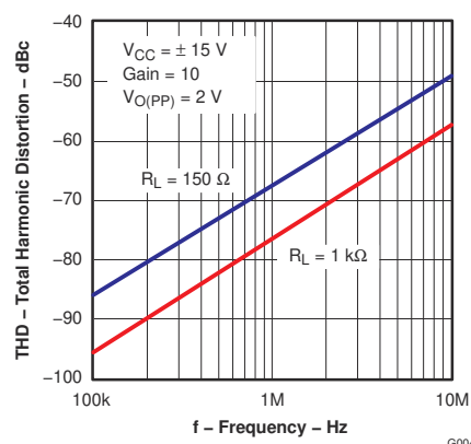
图 5-33. Total Harmonic Distortion vs Frequency
