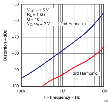
图 5-37. Distortion vs Frequency
