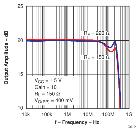
图 5-41. Output Amplitude vs Frequency
