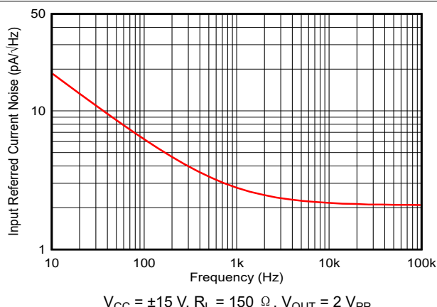
图 5-12. Input-Referred Current Noise vs Frequency
