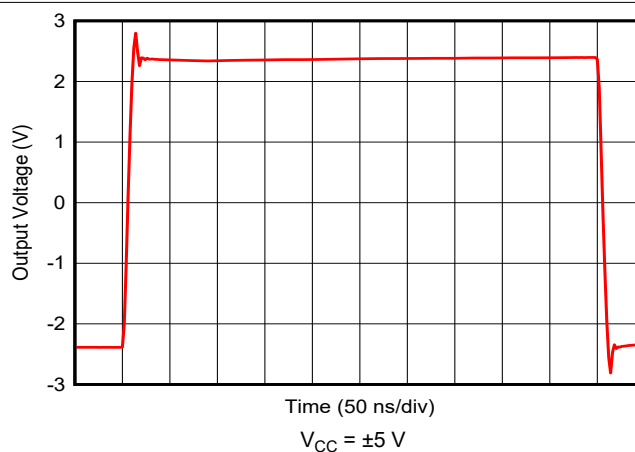
图 5-22. 5-V Step Response
