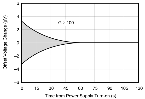
图 5-8. Offset Voltage Warm-up vs Time
