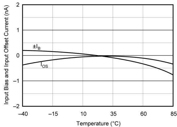
图 5-9. Input Bias and Input Offset Current vs Temperature
