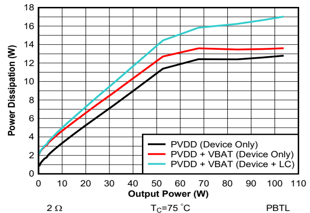
图 7-35. Power Dissipation vs Output Power - PBTL - 2 \Omega
