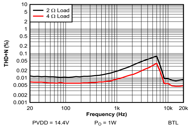
图 7-3. THD+N vs Frequency - 14.4 V
