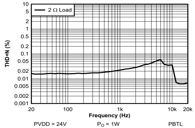
图 7-31. THD+N vs Frequency - PBTl - 24 V
