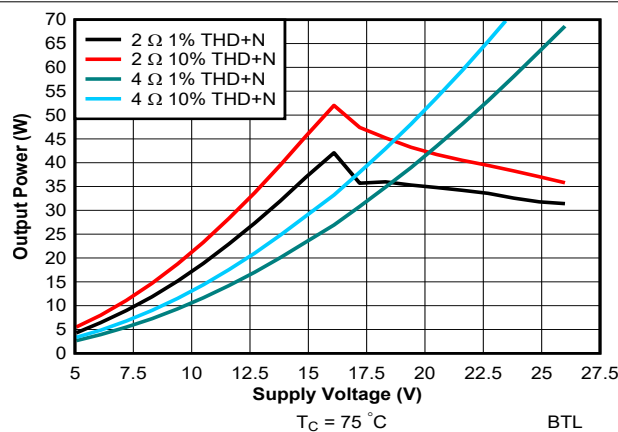
图 7-5. Output Power vs Supply Voltage
