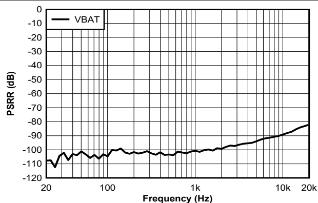
P_O = 1\text{ W} VBAT = 14.4\text{ V} + 1\text{ V}_{RMS} BTL 图 7-17. PSRR vs Frequency - VBAT Only
