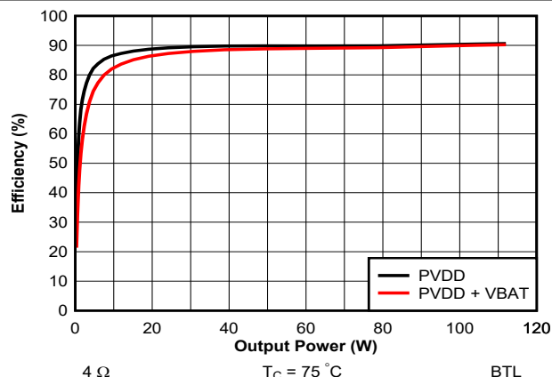
图 7-22. Efficiency vs Output Power - 4 Ω - 384 kHz
