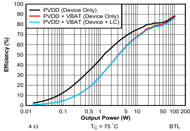
图 7-7. Efficiency vs Output Power - 14.4 V - 4 Ω (Zoomed)
