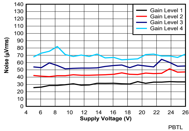
图 7-36. Noise vs Supply Voltage - PBTL
