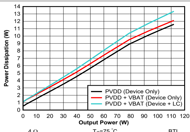
图 7-24. Power Dissipation vs Output Power - 4 Ω - 384 kHz
