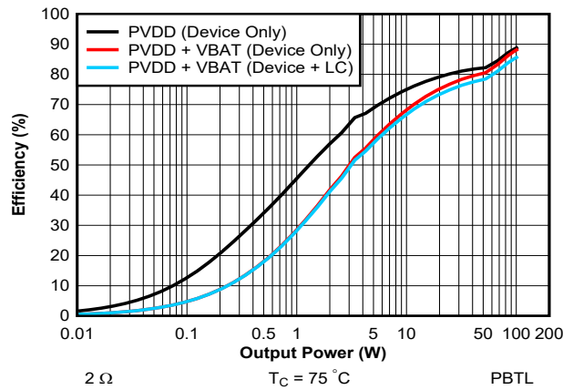
图 7-34. Efficiency vs Output power - PBTL - 2 \Omega (Zoomed)
