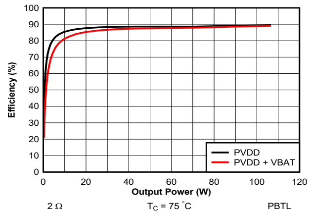
图 7-40. Efficiency vs Output Power - PBTL - 2 \Omega - 384 kHz
