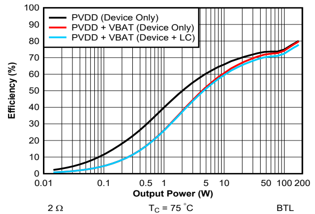
图 7-10. Efficiency vs Output Power - 14.4 V - 2 Ω (Zoomed)
