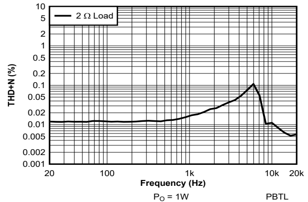
图 7-38. THD+N vs Frequency - PBTL - 384 kHz
