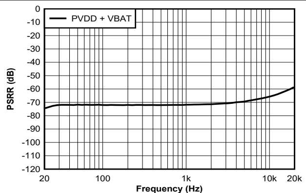
P_O = 1\text{ W} PVDD = VBAT = 14.4\text{ V} + 1\text{ V}_{RMS} BTL 图 7-18. PSRR vs Frequency - PVDD + VBAT
