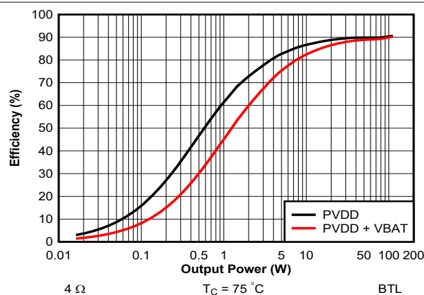
图 7-23. Efficiency vs Output Power - 4 Ω - 384 kHz (Zoomed)
