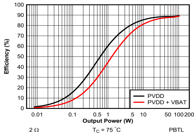
图 7-41. Efficiency vs Output Power - PBTL - 2 \Omega - 384 kHz (Zoomed)
