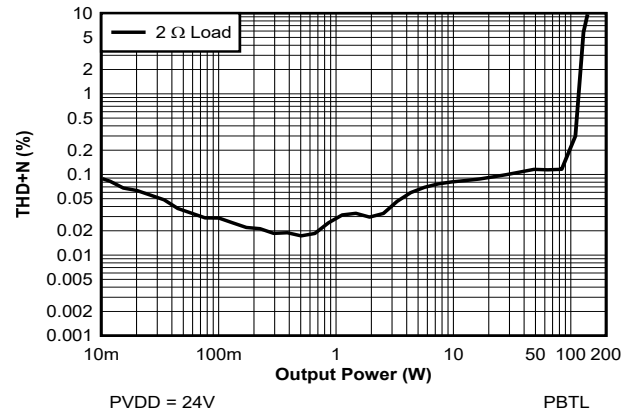
图 7-29. THD+N vs Power - PBTl - 24 V
