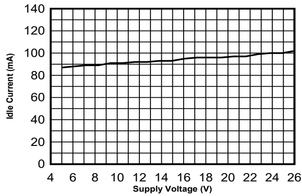
图 7-13. VBAT Idle Current vs Supply Voltage
