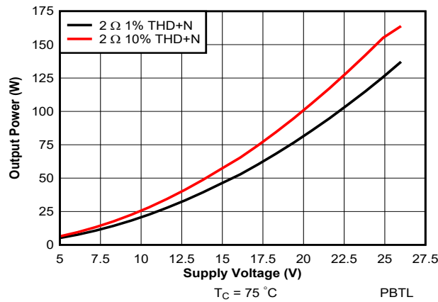
图 7-39. Output Power vs Supply Voltage - PBTL - 384 kHz
