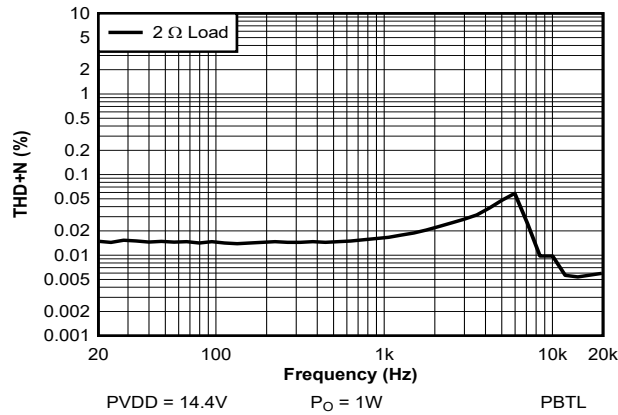
图 7-30. THD+N vs Frequency - PBTl - 14.4 V
