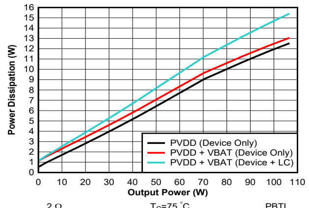
图 7-42. Power Dissipation vs Output Power - PBTL - 2 \Omega - 384 kHz
