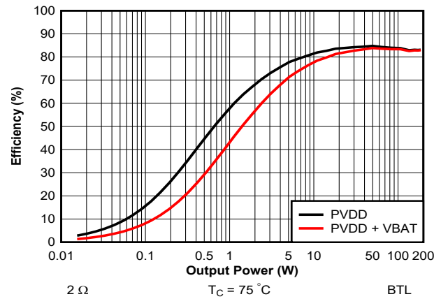
图 7-26. Efficiency vs Output Power - 2 \Omega - 384 kHz (Zoomed)
