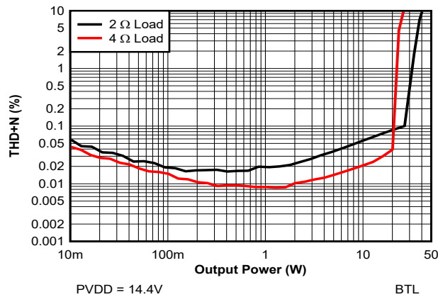
图 7-1. THD+N vs Power - 14.4V
