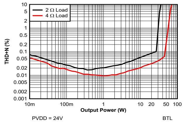
图 7-2. THD+N vs Power - 24V
