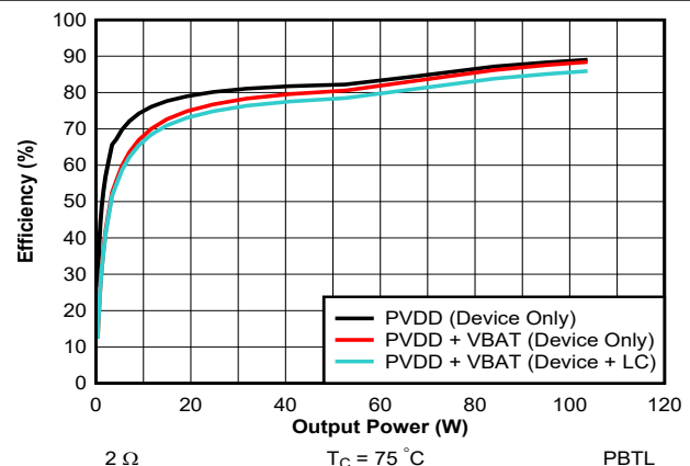
图 7-33. Efficiency vs Output Power - PBTl - 2 \Omega
