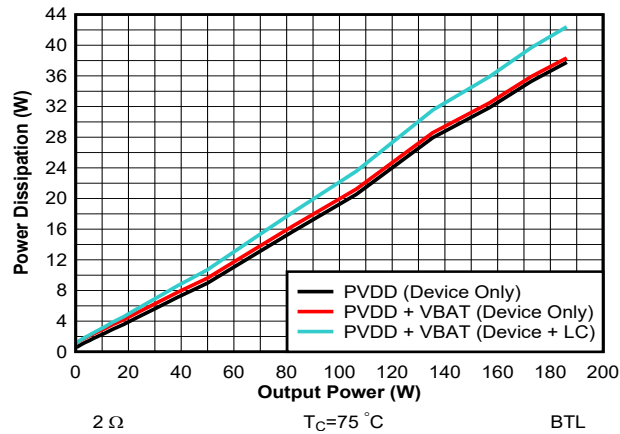
图 7-27. Power Dissipation vs Output Power - 2 \Omega - 384 kHz
