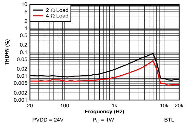
图 7-4. THD+N vs Frequency - 24 V
