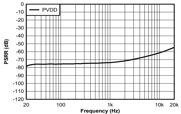
P_O = 1\text{ W} PVDD = 14.4\text{ V} + 1\text{ V}_{RMS} BTL 图 7-16. PSRR vs Frequency - PVDD Only
