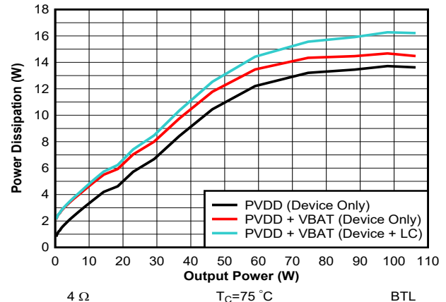
图 7-8. Power Dissipation vs Output Power - 14.4 V - 4 Ω
