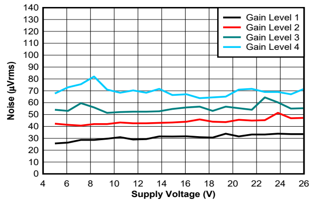
图 7-14. Noise vs Supply Voltage
