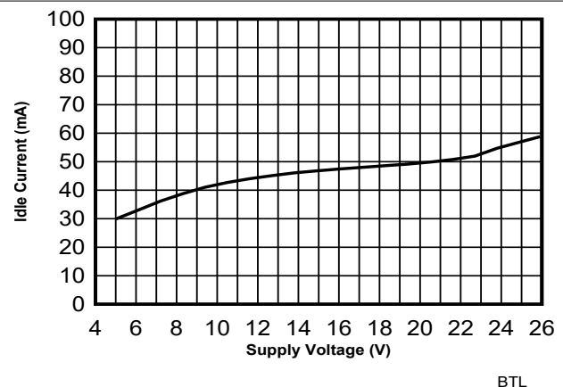
图 7-12. PVDD Idle Current vs Supply Voltage
