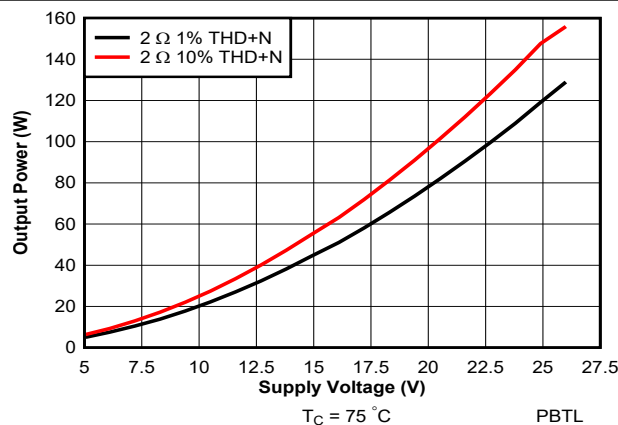
图 7-32. Output Power vs Supply Voltage - PBTl
