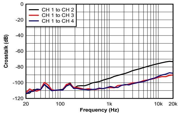
图 7-15. Crosstalk vs Frequency
