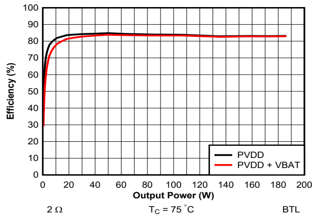
图 7-25. Efficiency vs Output Power - 2 \Omega - 384 kHz
