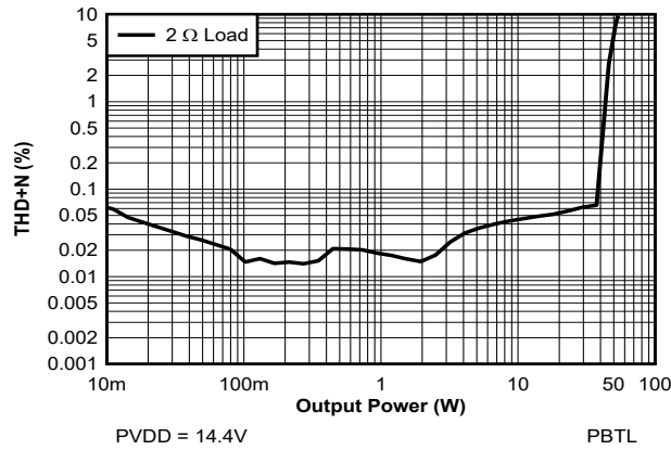
图 7-28. THD+N vs Power - PBTl - 14.4V
