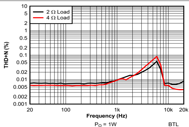
图 7-20. THD+N vs Frequency - 384 kHz
