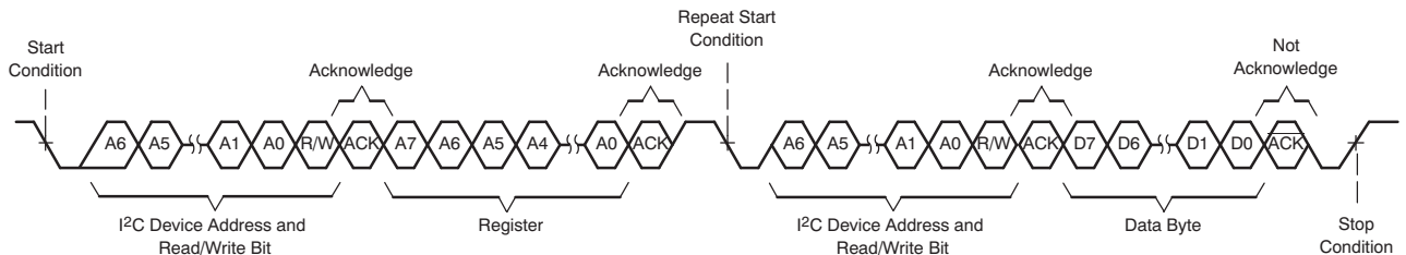
Figure 92. I 2 C Single-Byte Read Transfer
