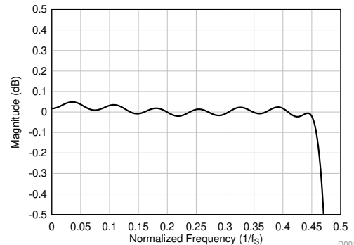
Figure 45. Linear Phase Decimation Filter Pass-Band Ripple
