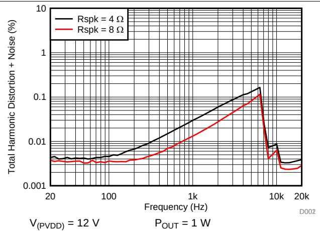
图 8. THD+N vs Frequency
