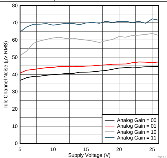
图 27. A-Weighted Idle Channel Noise vs Supply Voltage
