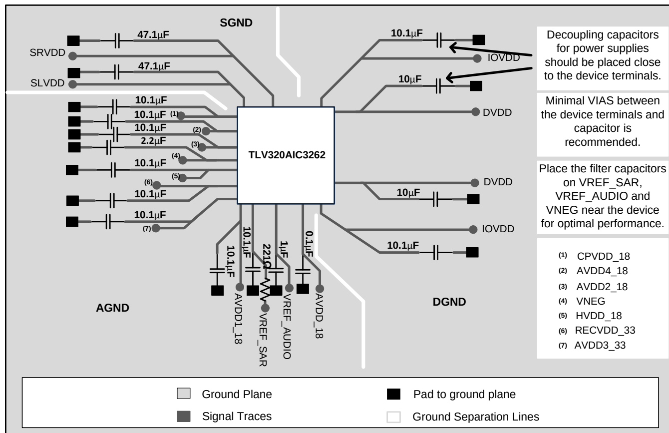
Figure 38. Power Layer
