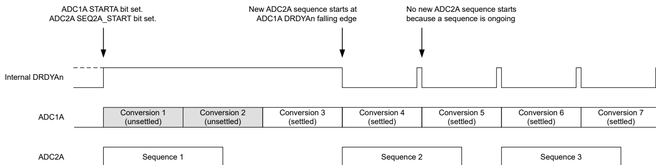
图 9-23. Synchronizing ADC1A Conversions and ADC2A Sequence Starts
