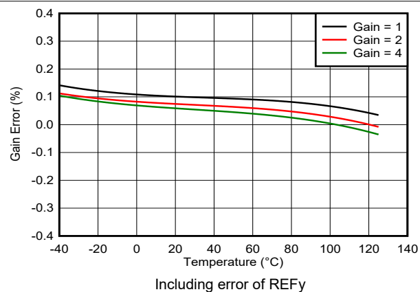
图 7-11. ADC2y Gain Error vs Temperature
