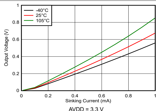
图 7-34. Analog GPIO Pin Output Voltage vs Sinking Current
