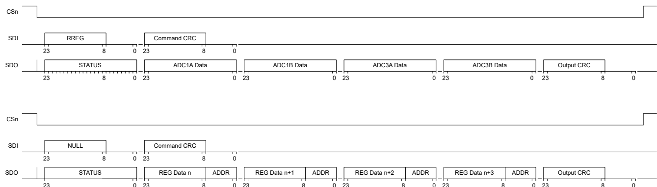
图 9-30. Bit Alignment, 24-Bit Word Size, RREG Command
