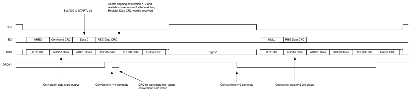
图 9-45. DRDYn Pin Behavior: Setting the STARTy Bit and Reading Conversion Data While New Conversions Complete
