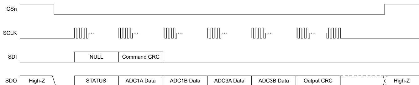
图 9-28. Typical Communication Frame
