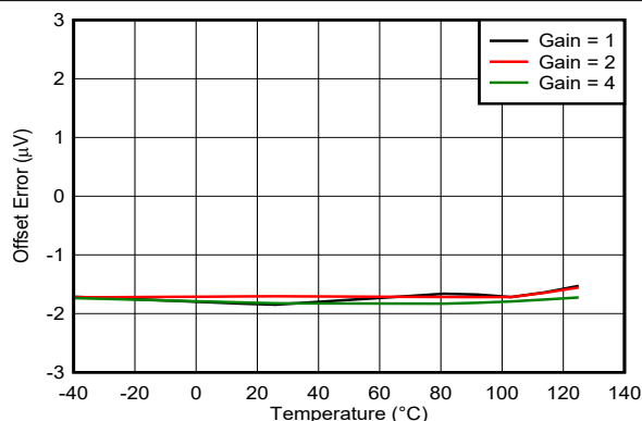
图 7-15. ADC3y Offset Error vs Temperature
