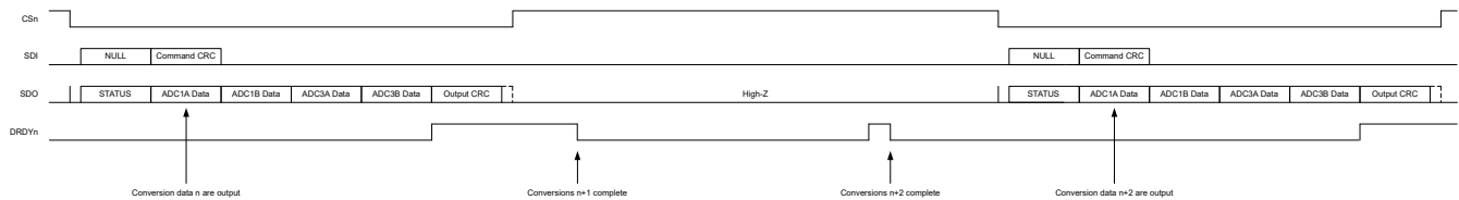
图 9-43. DRDYn Pin Behavior: Missed Reading Intermediate Conversion Results
