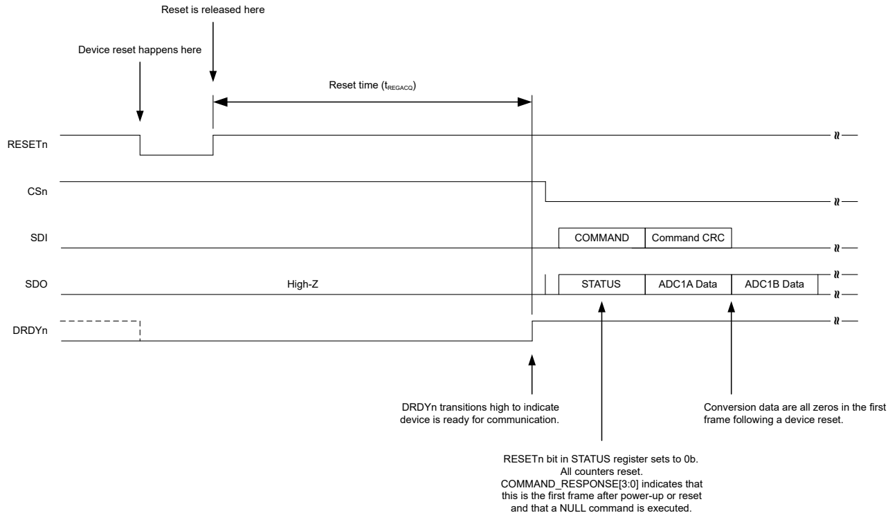
图 9-27. DRDYn Pin Behavior After Device Reset
