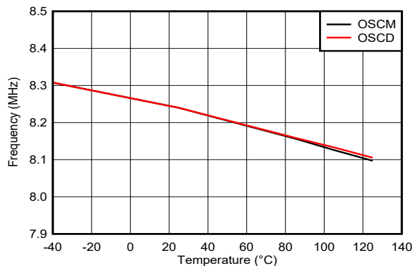
图 7-21. OSCM and OSCD Frequency vs Temperature
