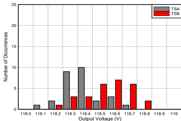
图 7-26. Temperature Sensor Output Voltage Histogram
