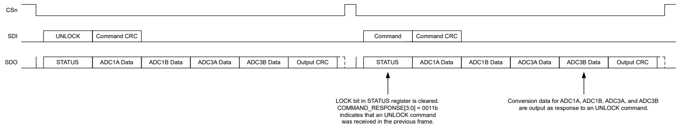
图 9-34. UNLOCK Command Frame
