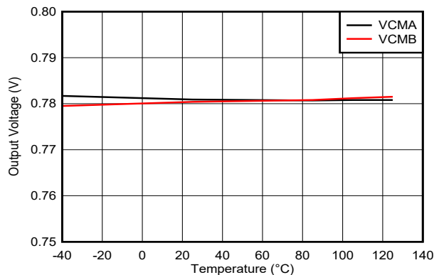
图 7-38. VCMY Output Voltage vs Temperature
