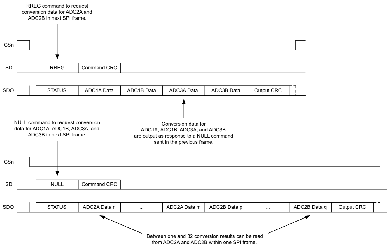
图 9-38. Reading Conversion Data From ADC1A, ADC1B, ADC2A, ADC2B, ADC3A, and ADC3B Within Two SPI Frames
