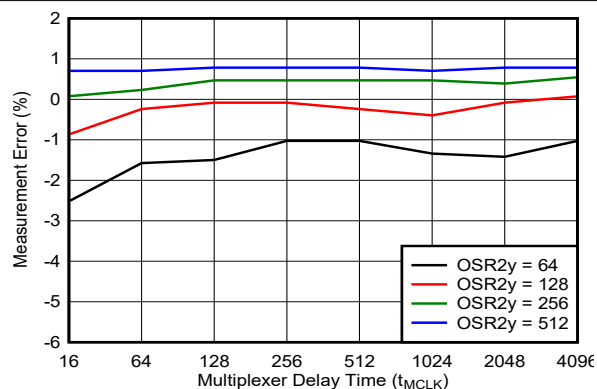
图 7-32. ADC2y Supply Voltage Readback Measurement Accuracy
