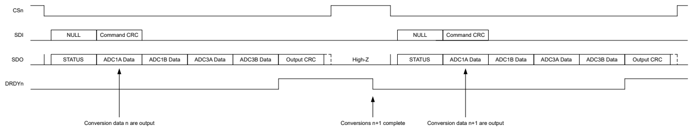
图 9-39. DRDYn Pin Behavior: Reading All Conversion Data Before New Conversions Complete
