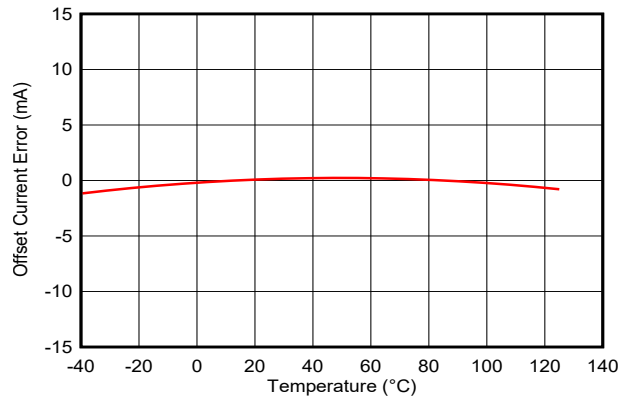
图 10-2. Offset Current Error vs Temperature (ADC1A, ADC1B)
