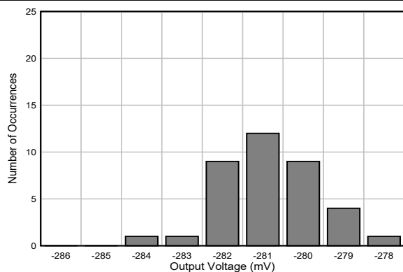
图 7-28. Test DACy Output Voltage Histogram
