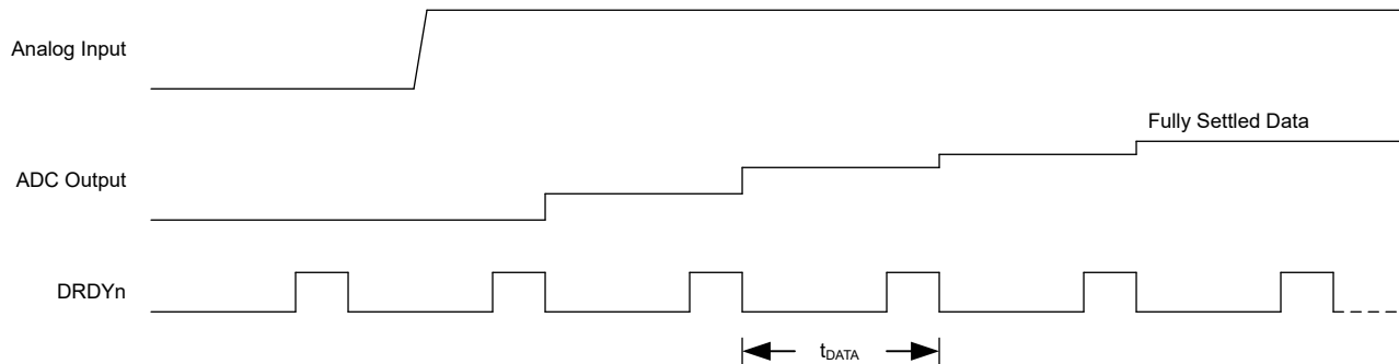
图 9-18. SINC3 Filter Behavior During Input Step Change
