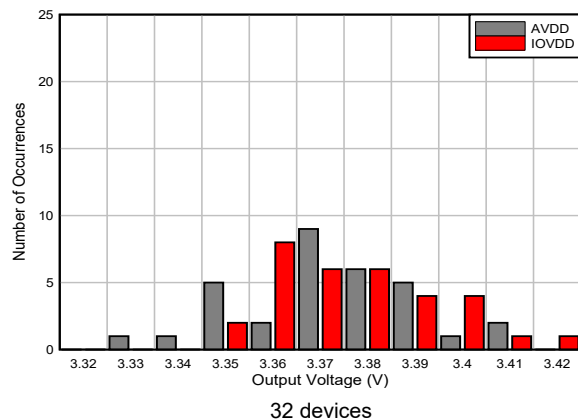
图 7-39. AVDD and IOVDD LDO Output Voltage Histogram
