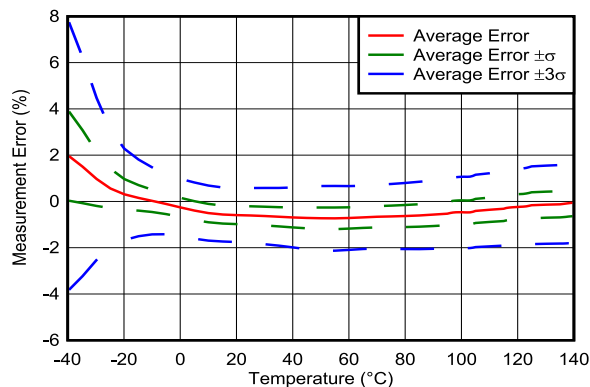
图 7-27. Temperature Sensor Measurement Error vs Ambient Temperature
