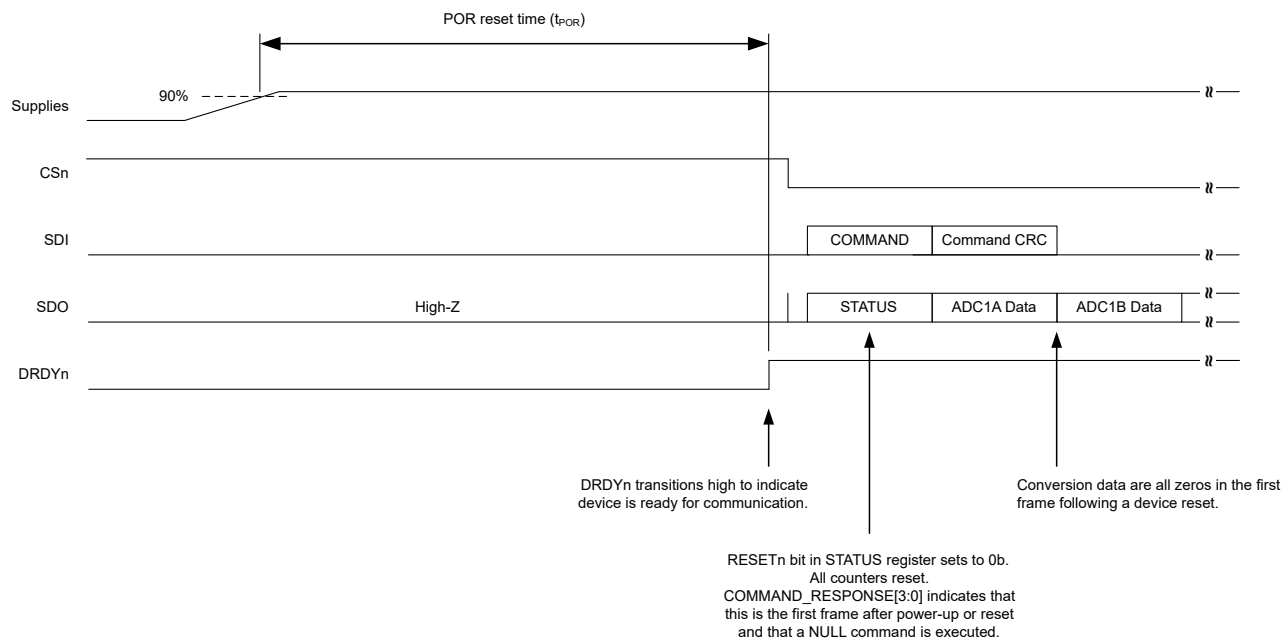
图 9-26. DRDYn Pin Behavior After POR
