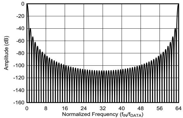
图 9-4. Sinc3 Filter Frequency Response to f_{MOD} (OSR = 64)
