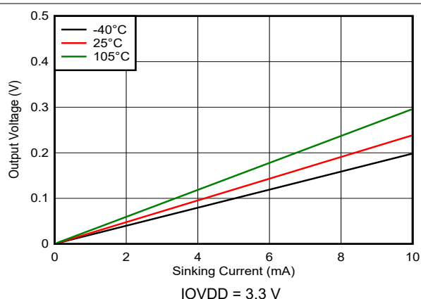
图 7-36. Digital Pin Output Voltage vs Sinking Current
