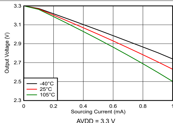
图 7-35. Analog GPIO Pin Output Voltage vs Sourcing Current
