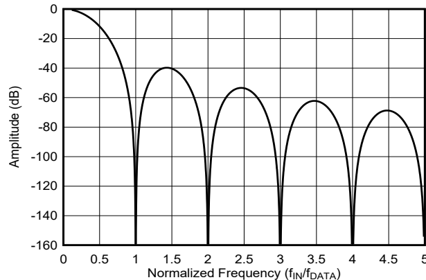
图 9-3. Sinc3 Filter Frequency Response
