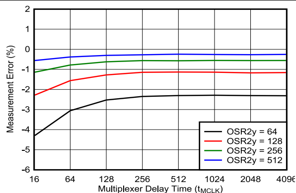
图 7-33. ADC2y Supply Voltage Readback Measurement Accuracy
