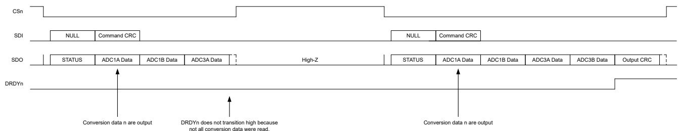
图 9-41. DRDYn Pin Behavior: Incomplete Read of Conversion Data Followed by Complete Read of Same Conversion Data
