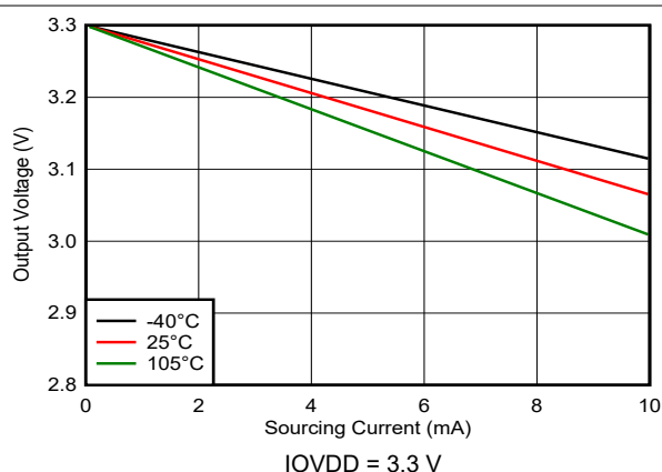
图 7-37. Digital Pin Output Voltage vs Sourcing Current
