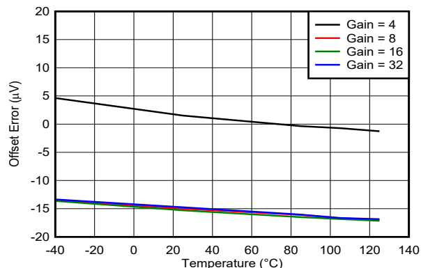
图 7-3. ADC1y Offset Error vs Temperature
