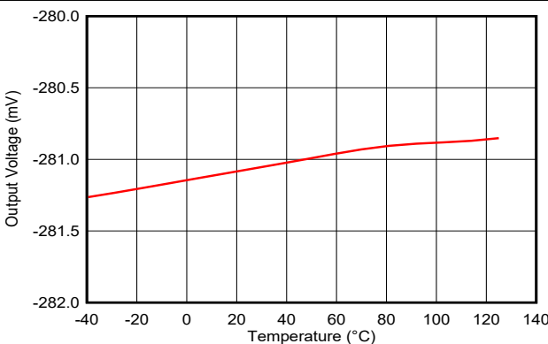
图 7-29. Test DACy Output Voltage vs Temperature
