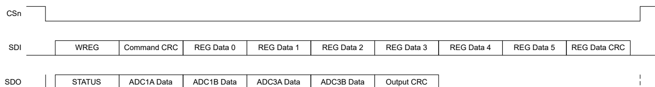
图 9-36. WREG Command Frame (Six Registers)
