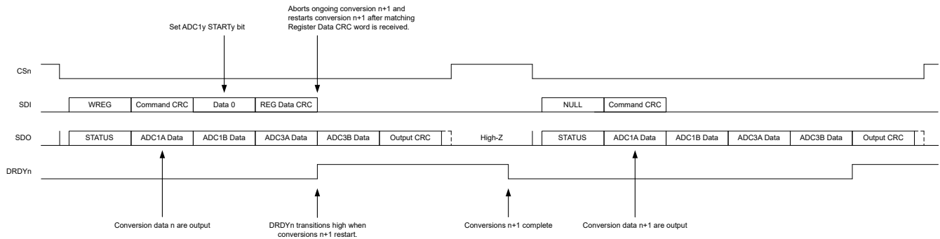
图 9-44. DRDYn Pin Behavior: Setting the STARTy Bit While Reading Conversion Data
