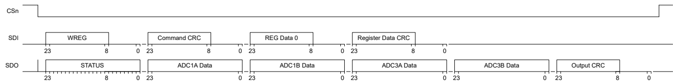
图 9-29. Bit Alignment, 24-Bit Word Size, WREG Command
