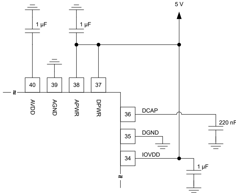
图 10-7. Single Regulated External 5-V Supply
