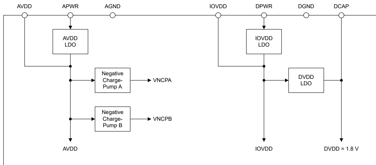
图 10-4. Power-Supply Architecture
