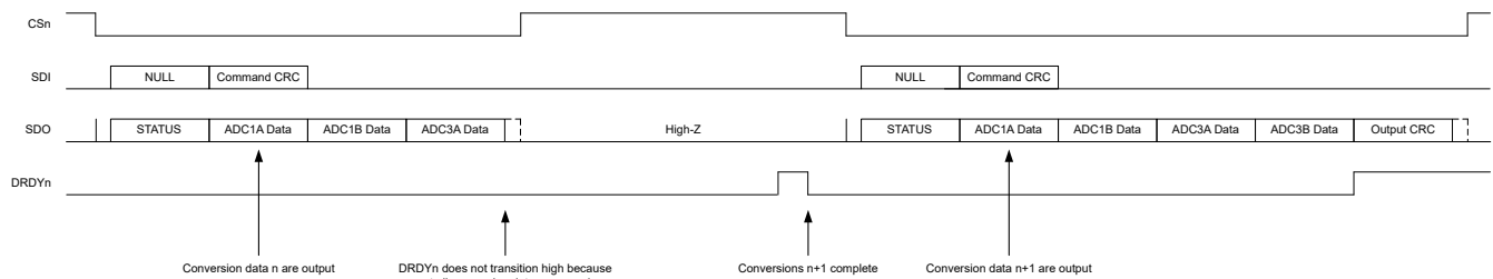
图 9-40. DRDYn Pin Behavior: Incomplete Read of Conversion Data Before New Conversions Complete
