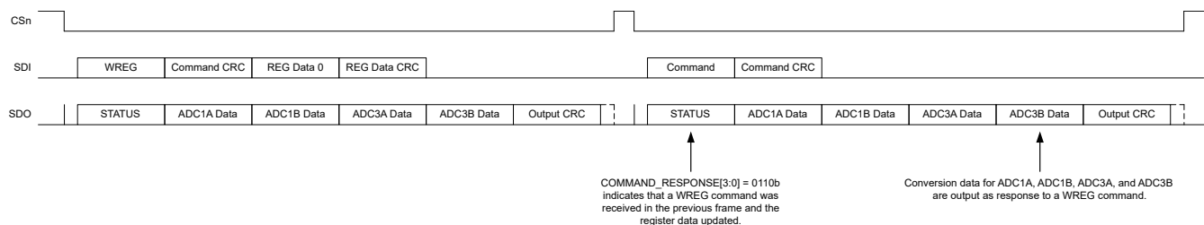
图 9-35. WREG Command Frame (Single Register)
