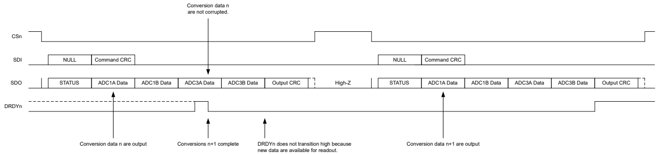
图 9-42. DRDYn Pin Behavior: Reading Conversion Data While New Conversions Complete
